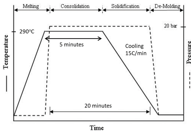
Fig. 2. Hot press consolidation profile
