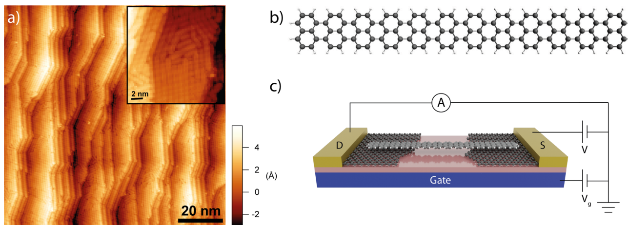
Figure 1. STM characterization and device geometry. (a) STM image of as-synthesized aligned 5-AGNR on a Au (788) surface ( V_s = -1.5 V, I_t = 0.06 nA). (b) Schematic of a 5-AGNR. (c) Schematic of the 5-AGNR bridging a graphene nanogap and of the electrical transport measurement setup.
