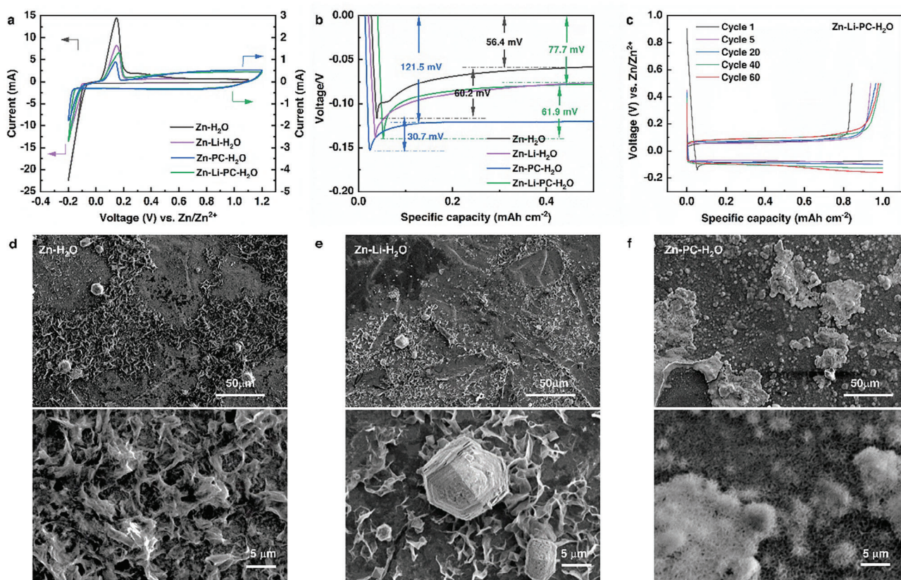
Figure 2. a) CV curves of \text{Ti}_3\text{C}_2\text{T}_x/\text{Zn} cell in Zn- \text{H}_2\text{O} , Zn-Li- \text{H}_2\text{O} , Zn-PC- \text{H}_2\text{O} , and Zn-Li-PC- \text{H}_2\text{O} electrolytes at a sweep rate of 0.5 \text{ mV s}^{-1} . b) Voltage profiles (1st cycle) and corresponding nucleation overpotential values of \text{Ti}_3\text{C}_2\text{T}_x/\text{Zn} cell at a current density of 1 \text{ mA cm}^{-2} in different electrolytes. c) Charge/discharge curves of \text{Ti}_3\text{C}_2\text{T}_x/\text{Zn} cell in Zn-Li-PC- \text{H}_2\text{O} (Capacity: 1 \text{ mAh cm}^{-2} , current density: 1 \text{ mA cm}^{-2} ). SEM images of \text{Ti}_3\text{C}_2\text{T}_x electrode after plating 1 \text{ mAh cm}^{-2} of Zn at 1 \text{ mA cm}^{-2} in d) Zn- \text{H}_2\text{O} electrolyte and e) Zn-Li- \text{H}_2\text{O} electrolyte f) Zn-PC- \text{H}_2\text{O} electrolyte.
