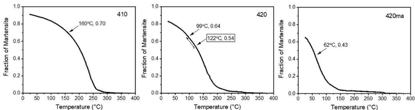
Fig. 3. Graphs showing the fraction of martensite formed during cooling as a function of temperature for alloys 410, 420 and 420ma.
