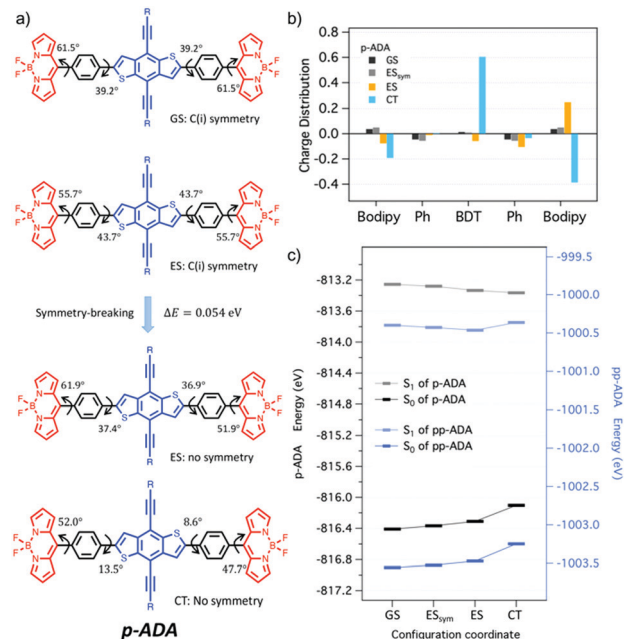
Fig. 5 Geometry optimization of the excited state. (a) Torsion angles in the geometry optimized ground state (GS), symmetrical excited state (ES sym ), asymmetrical excited state (ES) and charge transfer state (CT) of p-ADA . (b) Geometry-dependent charge distribution of the excited state as compared to the ground-state following the lowest vertical transition of p-ADA . (c) Energy levels of S_0 and S_1 corresponding to the geometries of GS, ES sym , ES and CT of p-ADA and pp-ADA .
