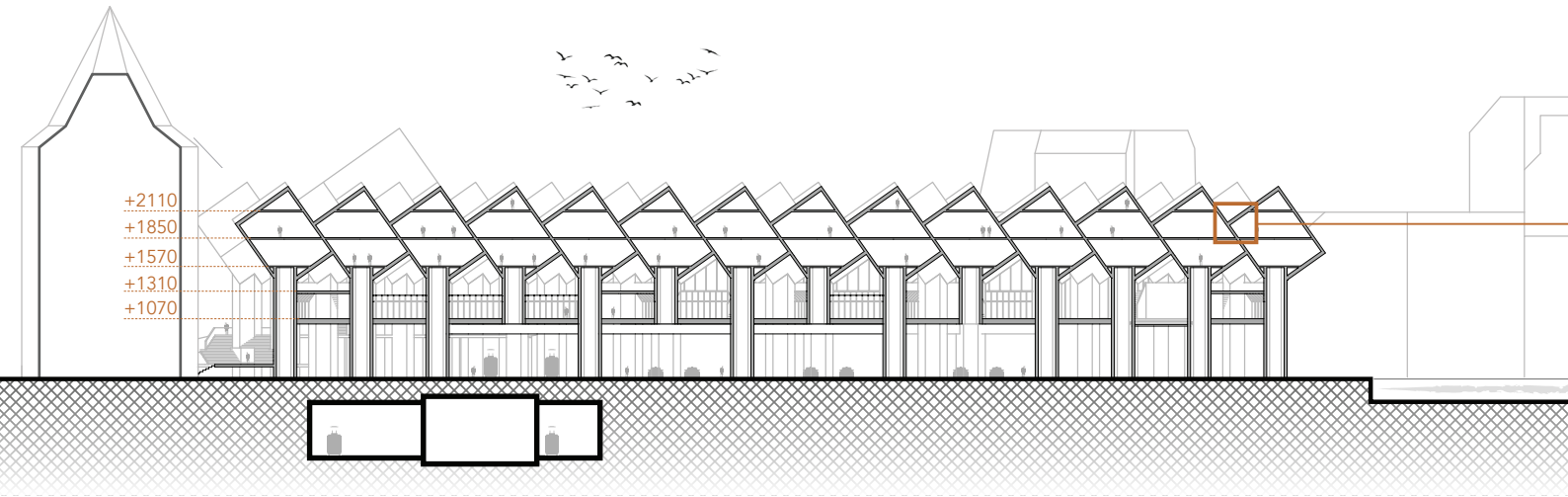
fig 10: section Overblaak
