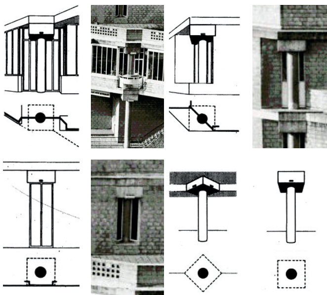
Figure 8: Study to the different column connections.
