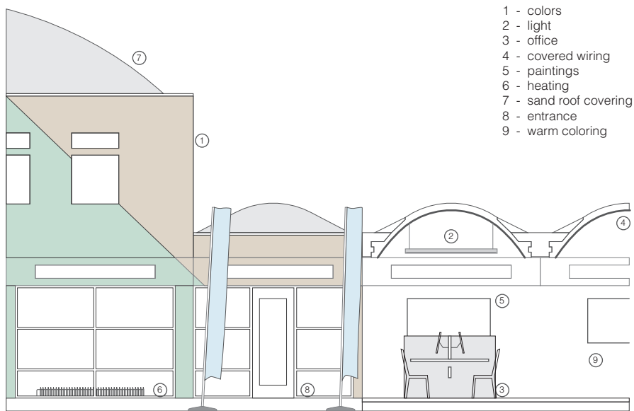
fig 29: Transformation diagram.
