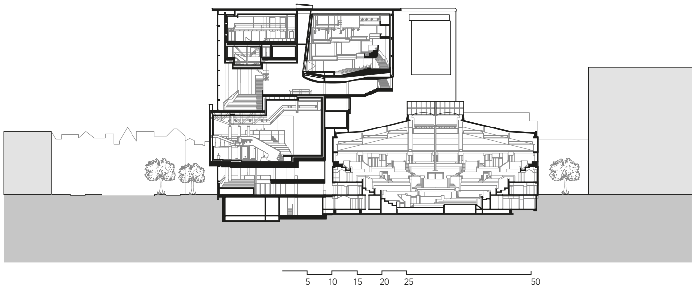
Figure 13: Section of the music palace Tivoli Vredenburg.
