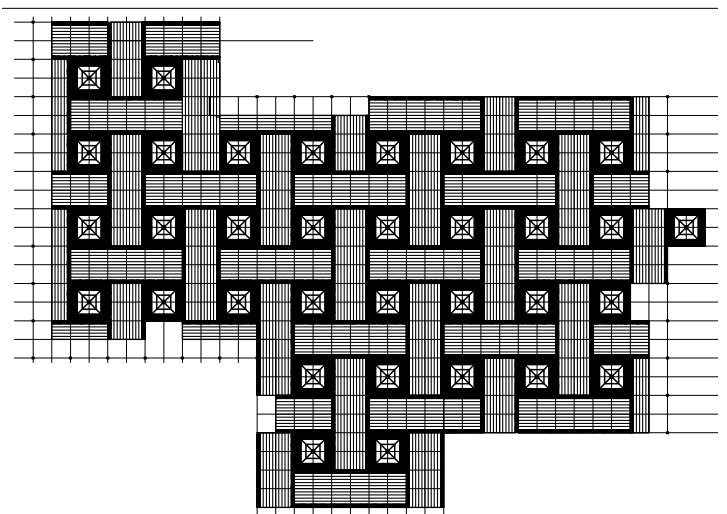
Fig 21. Roofplan drawing
