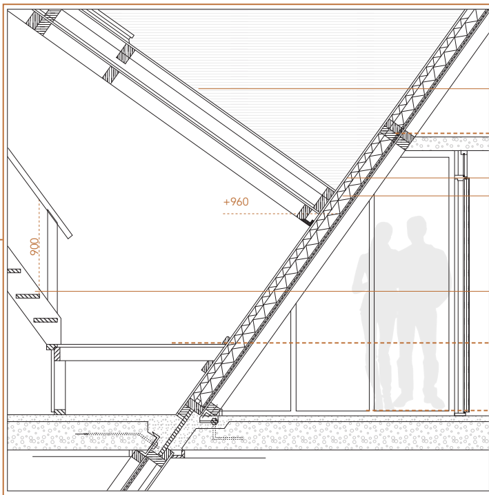
fig 12: Cube house detail
