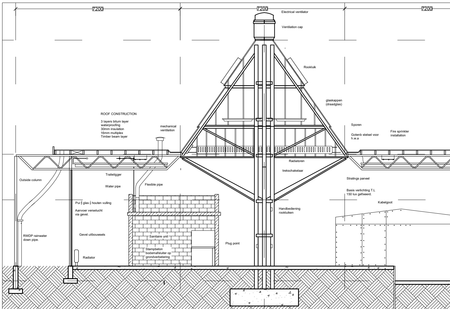
Fig 19. Scale 1:100 section.
