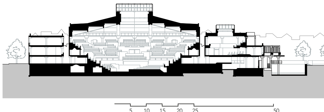
Figure 3: Section of the music centre.
