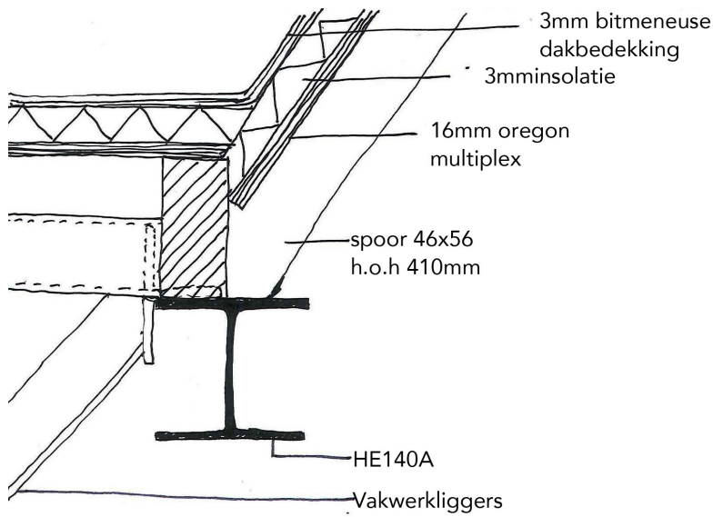
Fig 20. detail section
