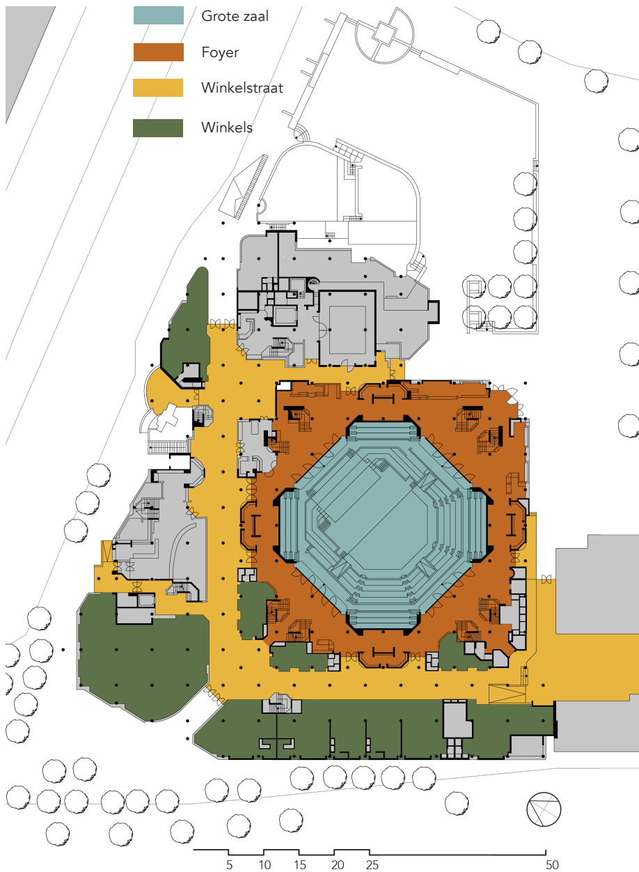
Figure 4: Floorplan of the ground floor with function indication.
