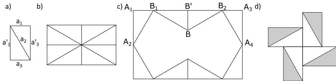
Fig. C.18. Representation of (a) the irregular chiral Rt structure ( Rt_I ) case where a_1 = a_3 \neq a'_1 = a'_3 , and (b) the achiralised ( ARt_{I2} ) and copy-rotated two times ( 2CAR_{I2} ) undeployed and (c) deployed structures. Representation (d) of the copy-rotation of Rt_{I4} , the irregular structure presents a topology close to Mr_4 , where the triangles in gray are rotating and the white ones are fixed.
