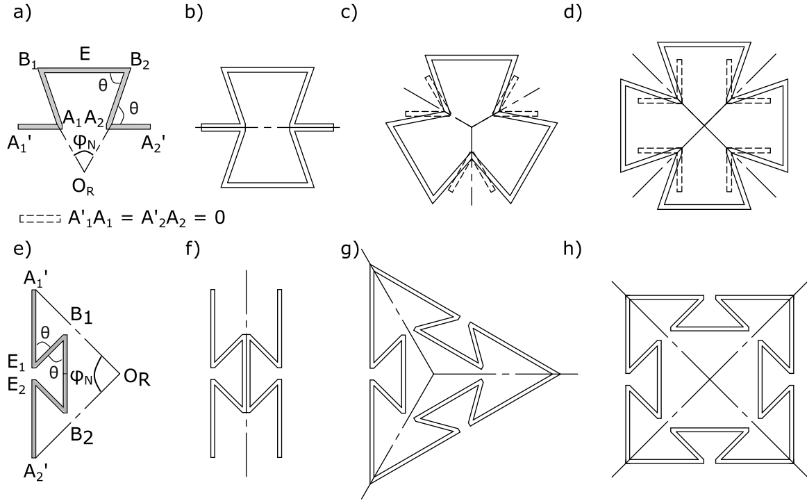
Fig. 7. Topological representation of the classical “puzzle tiles” auxetic achiral metamaterials, with (a) the construction of the center of rotation O_R , the representation of the undepleted (top) and depleted (bottom) case (b) 2Cpt where N=2 , (c) 3Cpt where N=3 , and (d) 4Cpt where N=4 . Topological representation of the reciprocal “puzzle tiles” auxetic achiral metamaterials, with (e) the construction of the center of rotation O_R , the representation of the undepleted cases (f) 2Rpt where N=2 , (g) 3Rpt where N=3 , and (h) 4Rpt where N=4 .
