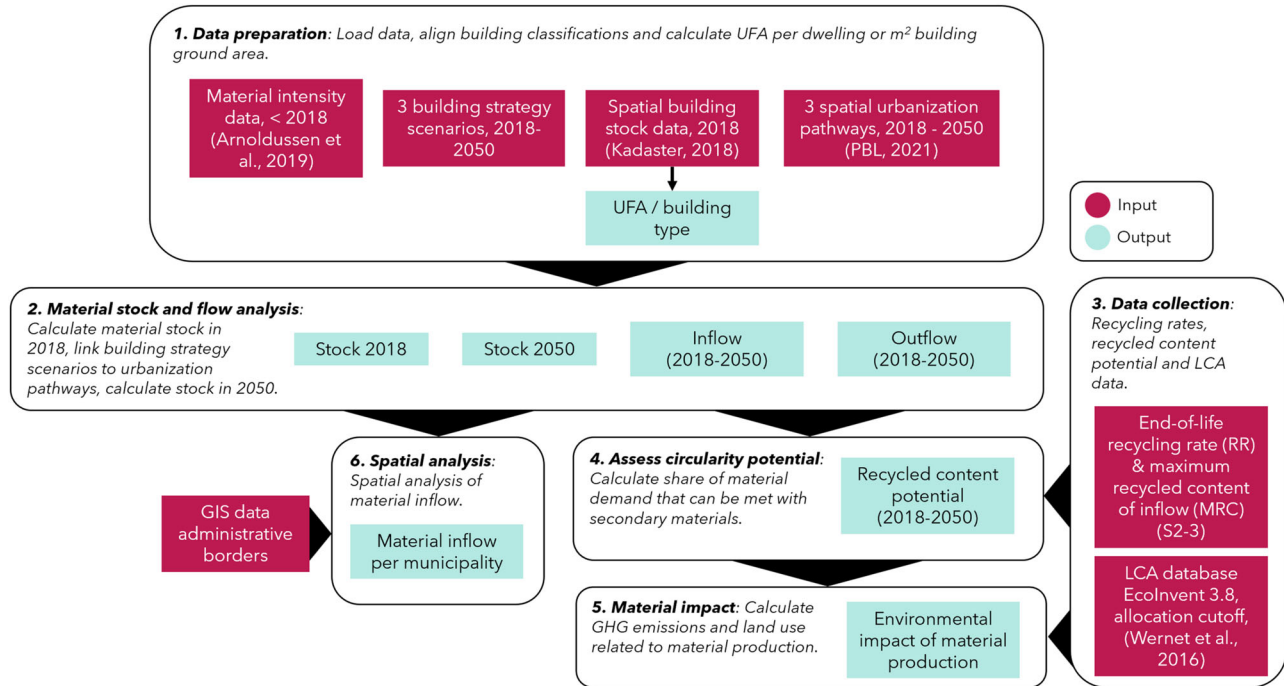
FIGURE 1 Model overview
