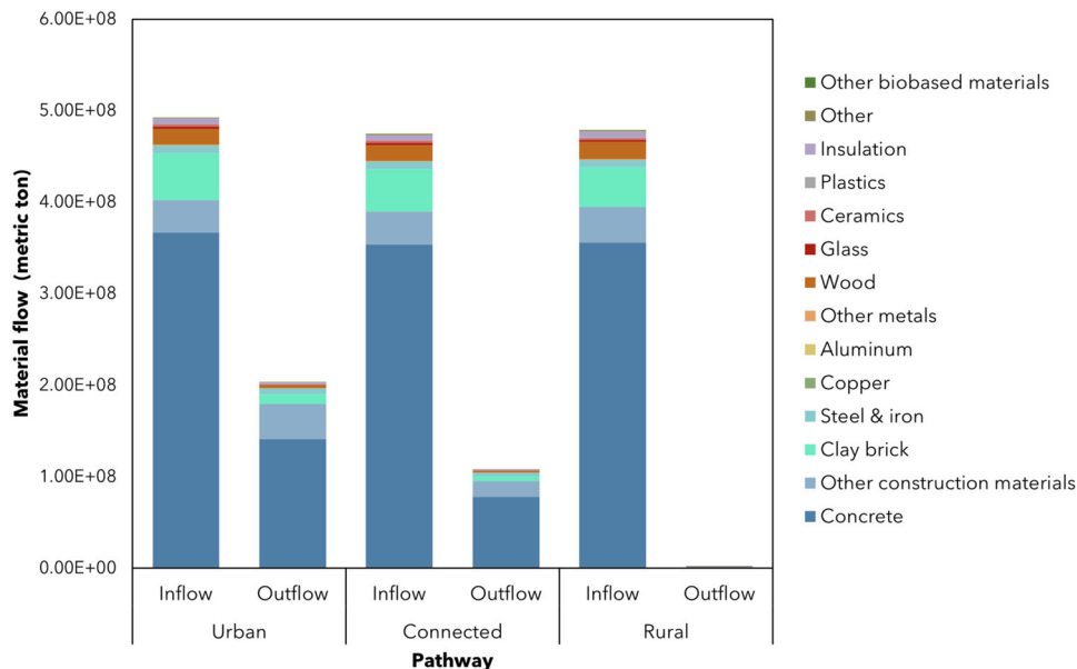
FIGURE 3 Cumulative material inflow and outflow between 2018 and 2050 for the three urbanization pathways (Conventional building strategy). Underlying data for this figure can be found in Supporting Information S3.
