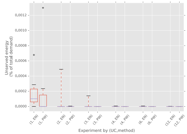
Fig. 4. Unserved energy in the NL system.
