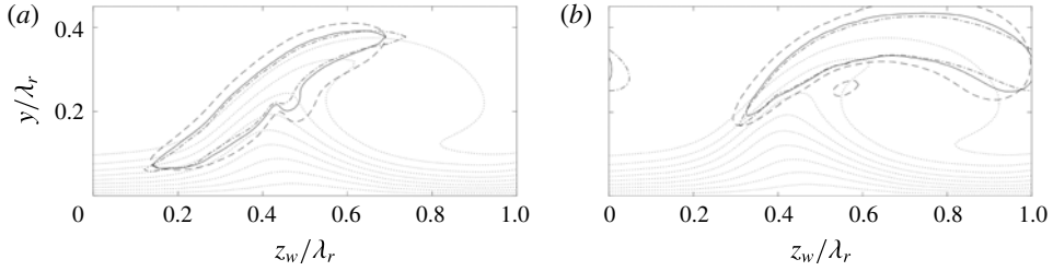
FIGURE 33. |\tilde{u}_w|/\max|\tilde{u}_w|=1/6 for Reynolds number: 10^{-0.8}Re (dashed line), nominal (solid) and 10^{0.8}Re (dash-dotted) for type I (a) and II (b). \overline{U}_w/\overline{U}_e levels 0.1, 0.2, ..., 0.9 (dotted).
