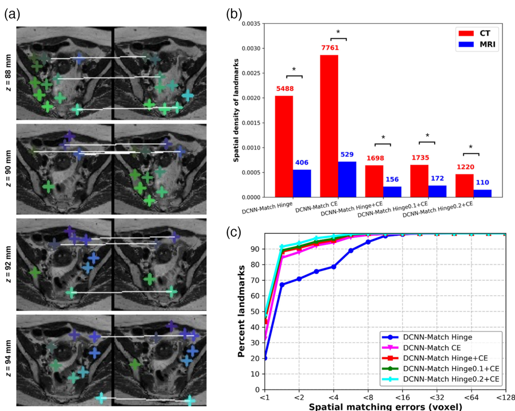
Fig. 13 Generalization results on the simulated deformations test set - MRI. (a) Predicted corresponding landmarks in the target and source MRI. Corresponding landmarks are shown with similar colored cross-hairs in the target and source images. Note that some of the landmarks match across slices following the underlying deformation in 3D. (b) Comparison of the spatial density of predicted landmarks (averaged over all patients) between simulated deformations test set - CT and simulated deformations test set - MRI for each DCNN-Match variant. The average number of predicted landmarks is shown in the text above bars. * indicates significant difference after Mann-Whitney U test. (c) Spatial matching errors of predicted landmark correspondences.
