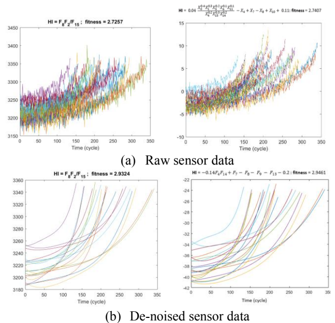
Figure 6. HIs constructed by (right column) the proposed and (left column) two-stage GP models, with (a) raw and (b) de-noised data using a validation (of 20% of training) set.
