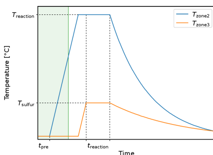
Figure 2.7: Representation of the temperature control aimed for within the atmospheric pressure CVD growth of WS 2 using the system depicted in Figure 2.6. The ideal profile of the temperature for both zone 2 ( T_{\text{zone2}} ) and zone 3 ( T_{\text{zone3}} ) are given. Here, perfect thermal isolation is assumed. The green shaded area illustrates the time period for which the flow rate is 500 sccm. After this, a reduced argon flow rate is supplied to the system.
