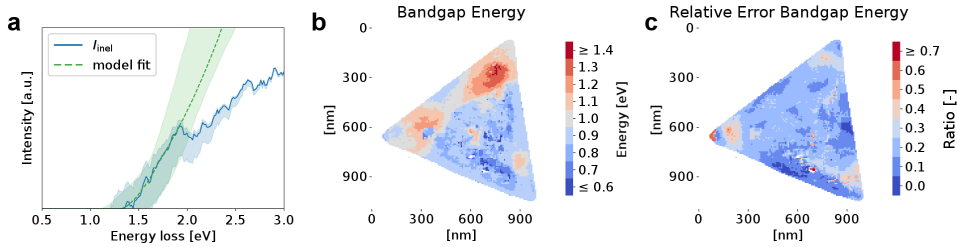
Figure 3.4: (a) The results of fitting Equation 3.1 to the onset of the subtracted inelastic EEL spectrum ( I_{inel} ). Here the exponent b was set to a fixed value of \frac{3}{2} due to the shape of the onset. The bands indicate the 68% confidence level uncertainties associated to the subtracted EEL spectrum and bandgap fit. (b) Spatially-resolved bandgap energy map corresponding to the twisted flakes specimen. (c) The relative uncertainties (68% confidence level intervals) associated to the bandgap energy map in (a). A mask has been applied to exclude substrate-only pixels and specimen pixels with a relative uncertainty exceeding 100%.
