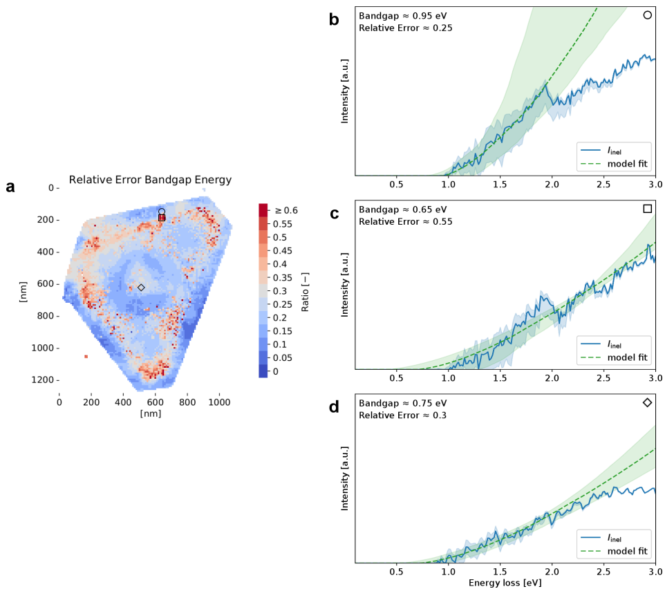
Figure B.1: The subtracted inelastic EEL spectra I_{inel} in three different regions (indicated in (a)) in the stacked flakes specimen: (b) at the edge (circle), (c) near the edge (square), and (d) in the center (diamond). The best-fit and uncertainty for the model of I_{inel} in the onset region, which are used to extract the bandgap energy, are also given. Note that some pixels near the edge regions exhibit additional structures in this onset region, which results in larger uncertainties in the bandgap energy determination.
