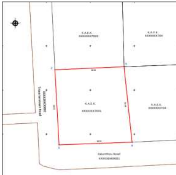
Figure 18a. Part of survey diagram depicting the parcel to be subdivided
