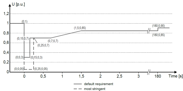
Fig. 1. LVRT Requirements, MV-connected SG in the Netherlands [3]
