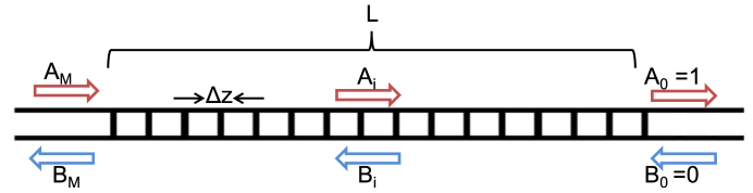
Fig. 1. Schematic view of the FBG structure.
