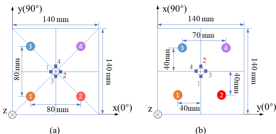
Figure 7: AE sensor distributions (circles) and locations of surface information extraction from DIC analysis (squares) for (a)PCLS-R(0//0) and (b)PCLS-R(0//90) specimens.
