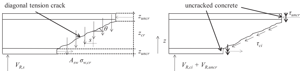
FIGURE 1 Possible shear transfer mechanism for a girder with stirrups in regions without flexural cracks
