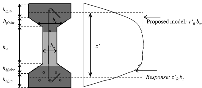
FIGURE 7 Distribution of shear stress times the cross-sectional or web width
