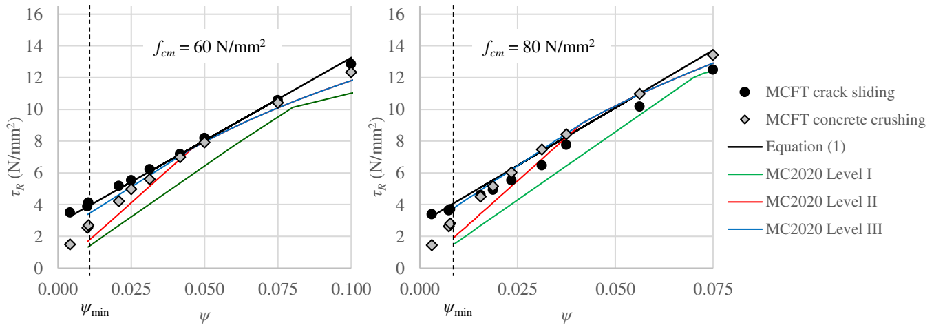
FIGURE 6 Shear resistance at \varepsilon_x = 0 versus \psi for f_{cm} = 60 \text{ N/mm}^2 and f_{cm} = 80 \text{ N/mm}^2
