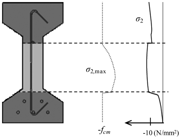
FIGURE 3 Stresses and maximum stresses in compression field at failure of HX1-A 14
