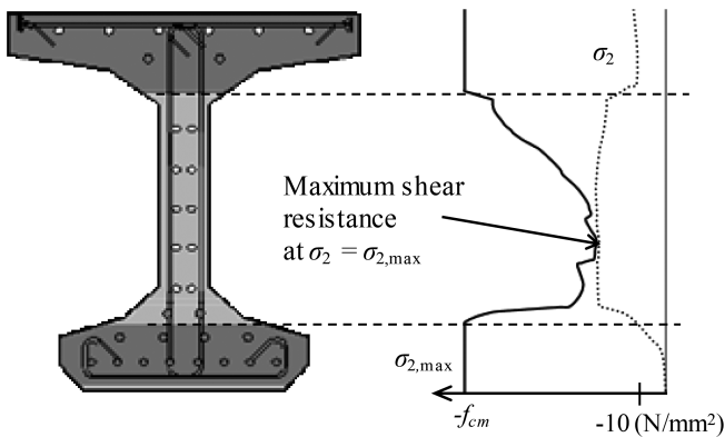
FIGURE 4 Stresses and maximum stresses in compression field at failure of HCP1TE 15
