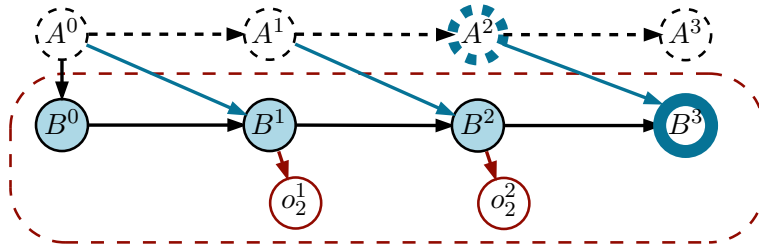
(c) The unrolled network G = \text{unroll}(G^0, G^\rightarrow) . To convert it to an IALM, the local-form initial belief b_i^{l,0}(B^0) and incoming influences I_{\rightarrow i}^{t+1}(A^t|B^0, \dots, B^t) need to be computed via inference. See text for further explanation.
