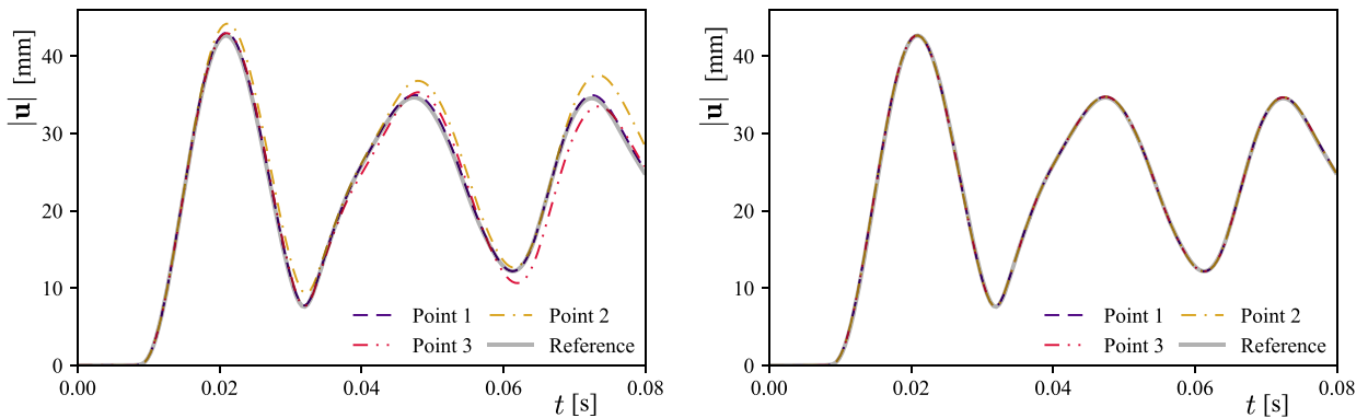
(a) Penalty formulation, with ghost-stabilized mass. (b) Nitsche formulation, with ghost-stabilized mass.
