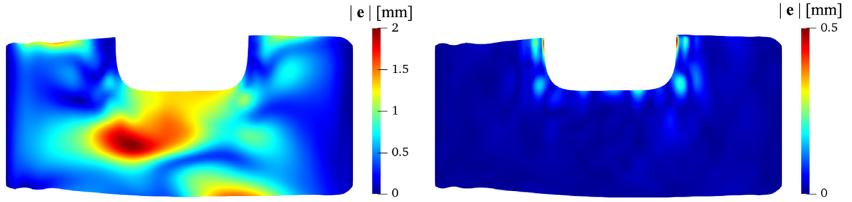
(a) Penalty formulation, with ghost-stabilized mass. (b) Nitsche formulation, with ghost-stabilized mass.
