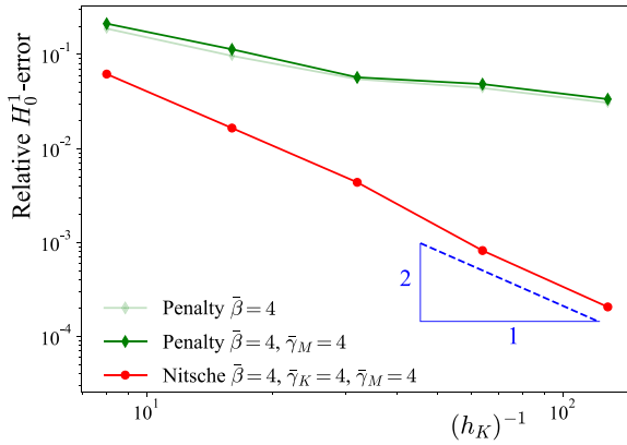
(c) H_0^1 -error, p = 2 .
