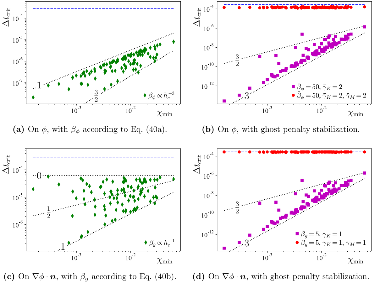
Fig. 15. Nitsche formulations for the fourth-order problem, for p = 2 : third, fourth and fifth row and second and third column in Tables 6–10. Critical time-step size dependency on the minimal element size fraction for 100 perturbations of the domain of Fig. 7.
