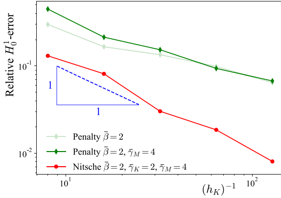
(a) H_0^1 -error, p = 1 .
