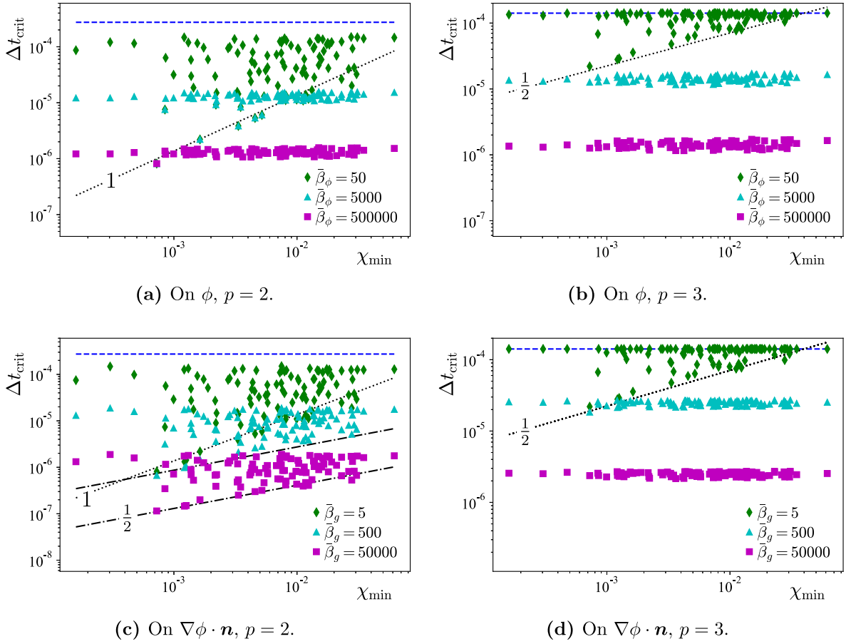
Fig. 11. Penalty formulations without ghost-stabilized mass for the fourth-order problem: second and fourth row and second column in Tables 6–10. Critical time-step size dependency on the minimal element size fraction for 100 perturbations of the domain of Fig. 7.
