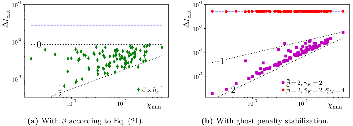
Fig. 14. Nitsche formulations for the second-order problem, for p = 1 : third and fourth row and second and third column in Tables 1–5. Critical time-step size dependency on the minimal element size fraction for 100 perturbations of the domain of Fig. 7.
