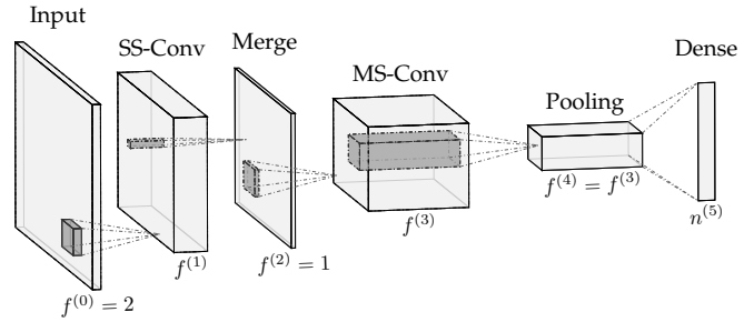
Fig. 5: Overview of the feedforward SNN architecture.
