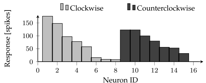
Fig. 11: Neural response of the individual neurons from the Dense layer trained in the rotating-disk sequence.
