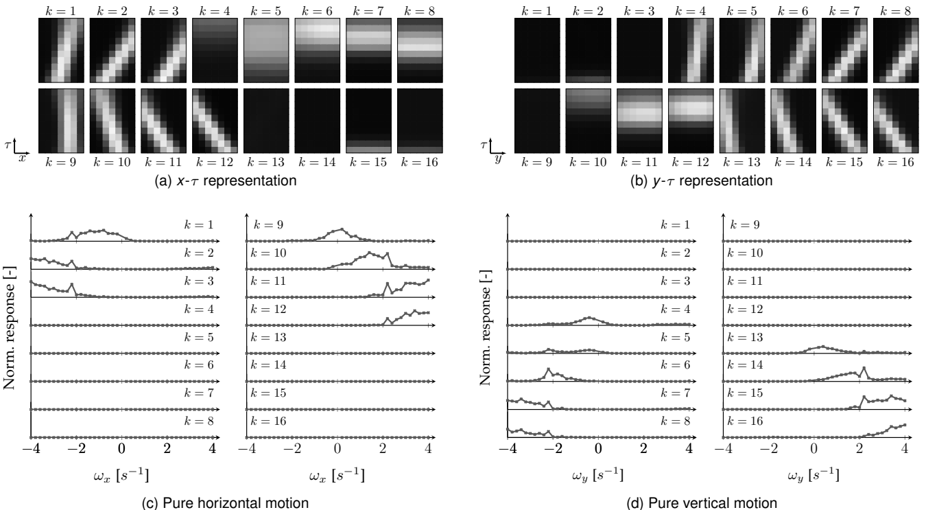
Fig. 7: Appearance (top) and neural response (bottom) of the sixteen spatiotemporal kernels learned from the checkerboard texture in the MS-Conv layer. Response plots are normalized by the maximum kernel response on the stimuli evaluated: 8.2763 spikes/ms by k = 11 for \omega_x = 4.0 \text{ s}^{-1} . Synaptic strength is encoded with brightness using the kernel formulation from Eq. (8), i.e. W^{\text{exc}} + \beta W^{\text{inh}} .
