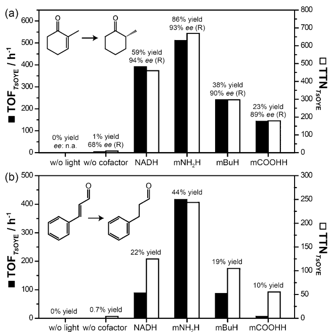
Figure 2. a) N-CD-sensitized photobiocatalytic reduction of (a) 2-methyl-2-cyclohexen-1-one (7 mM) and (b) trans -cinnamaldehyde (5 mM) by T_s\text{OYE} . Reaction conditions: N-CDs ( 0.10 \text{ mg mL}^{-1} ), M ( 25 \mu\text{M} ), substrate, cofactor (2 mM), T_s\text{OYE} ( 9 \mu\text{M} ), and \text{CaCl}_2 (5 mM) in a TEOA buffer (500 mM, pH 7.5) at 45^\circ\text{C} . Light intensity: 200 \text{ mW cm}^{-2} . Light source: a xenon lamp equipped with a 324 nm cut-on optical filter. TOF was determined after (a) 30 min and (b) 15 min of reaction. TTN and ee were determined after (a) 180 min and (b) 75 min of reaction.
