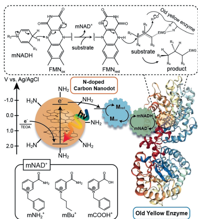
Scheme 1. Illustration of the photoenergy conversion into chemical energy by integrating photocatalysis and biocatalysis. Photoexcited electrons generated by N-doped carbon nanodots reduce the oxidized rhodium-based complex ( M_{ox} ) that regioselectively converts mNAD^+ into mNADH . Subsequently, the enzymatically active mNADH returns to its oxidized form after donating a hydride to a prosthetic group (i.e., flavin mononucleotide, FMN) in the old yellow enzyme. The reduced FMN transfers a hydride onto C\beta of a substrate while a Tyr-residue gives a proton onto C\alpha , resulting in the trans -specific reduction of an activated C=C bond. EWG: electron-withdrawing group.
