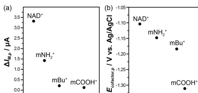
Figure 1. a) Comparison of changes in the cathodic peak current of 500 \mu M M ( \Delta I_{M,p} ) in the presence of 400 \mu M cofactor. b) Comparison of different reduction peak potentials of cofactors ( E_{cofactor,p} ). The electrochemical analysis was carried out in a phosphate buffer (100 mM, pH 7.5) at a scan rate of 50 \text{ mV s}^{-1} . Working electrode: a polished glassy carbon electrode.
