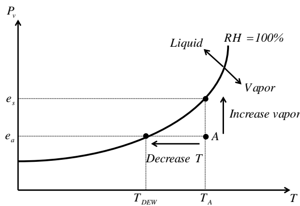
Figure 3. Graph of vapor pressure ( P_v ) against temperature ( T ), showing the position of saturated vapor pressure ( e_s ) and dewpoint temperature ( T_{DEW} ). RH = relative humidity.
