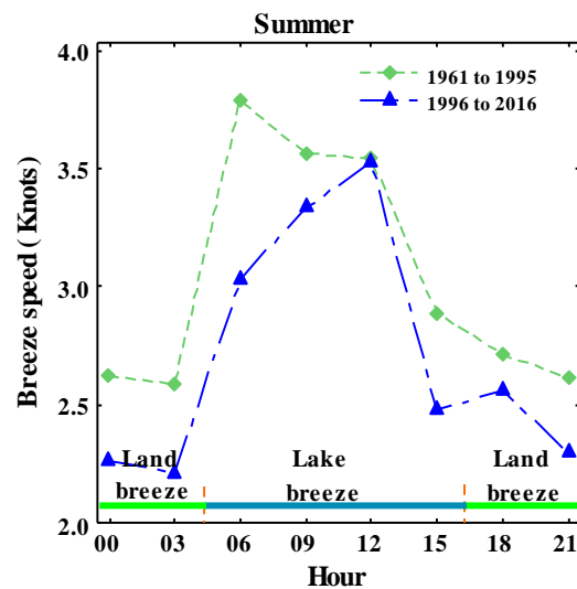
Figure 9. Speed of summer lake and land breezes at Urmia meteorological station in sub-periods with normal (1961–1995) and low level (1996–2016) in Lake Urmia.
