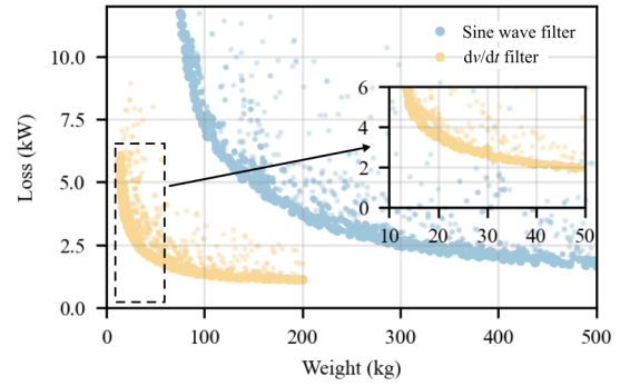
Fig. 7. MOO results of sine wave and dv/dt filters.
