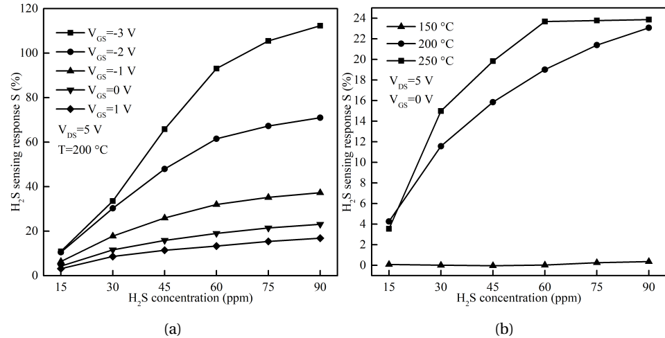
Figure 4.6: Hydrogen sulfide sensor sensing response at (a) various gate bias voltages and (b) at different temperatures.
