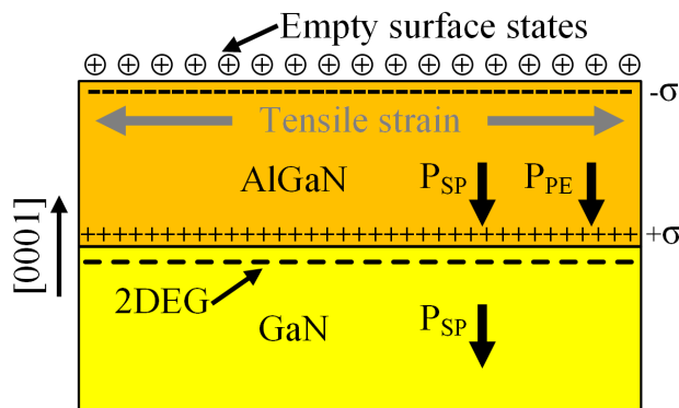
Figure 2.5: Orientation of polarization vectors at the Ga-face AlGaIn/GaN heterostructure with AlGaIn under tensile strain. Polarization induced charges ( \sigma ) are also indicated.
