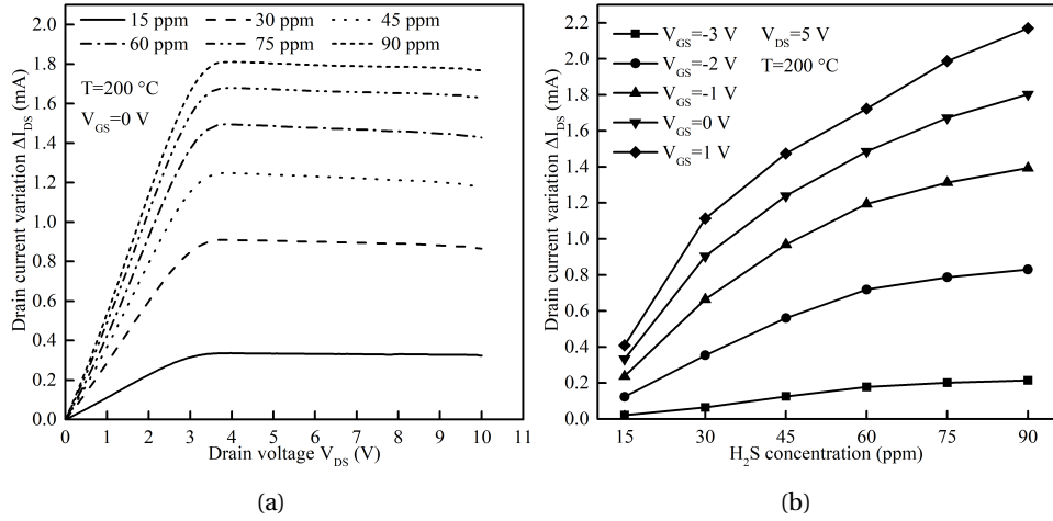
Figure 4.5: (a) Drain current variation ( \Delta I_{DS} ) as a function of drain-source ( V_{DS} ) voltage for different \text{H}_2\text{S} concentrations at 200\text{ }^\circ\text{C} , V_{GS}=0\text{ V} . (b) Drain current variation ( \Delta I_{DS} ) versus \text{H}_2\text{S} concentration at 200\text{ }^\circ\text{C} , V_{DS}=5\text{ V} .
