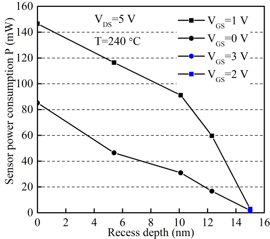
Figure 5.16: Power consumption values for sensors A–E at 240 °C and V_{DS}=5\text{ V} .
