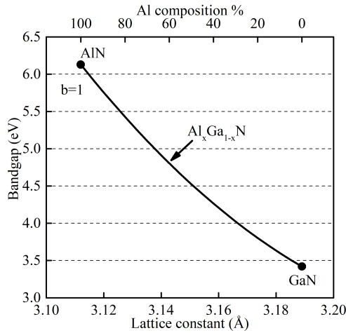
Figure 2.4: Variation of bandgap versus lattice constant and Al incorporation of AlGaIn alloy.
