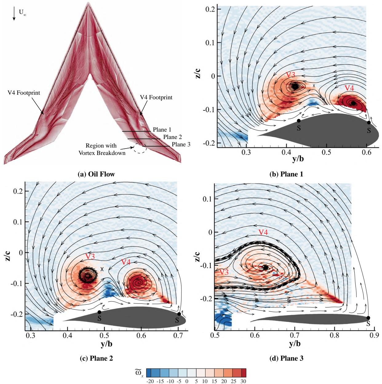
Fig. 13 Oil flow and normalized axial vorticity with cross-flow topology, viewed upstream at \alpha = 17.5^\circ , with Re_c = 8.0 \times 10^5 and M = 0.10 .
