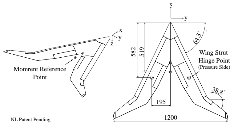
Fig. 3 Technical drawing of the modular wind tunnel model, based on the Flying V design by Laar [18, 19]. Dimensions are in mm.
