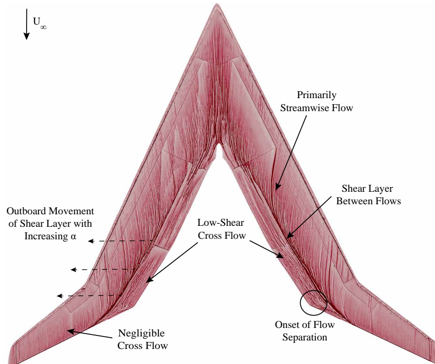
Fig. 7 Oil flow and annotated flow features at \alpha = 0.0^\circ , with Re_c = 8.0 \times 10^5 and M = 0.10 .
