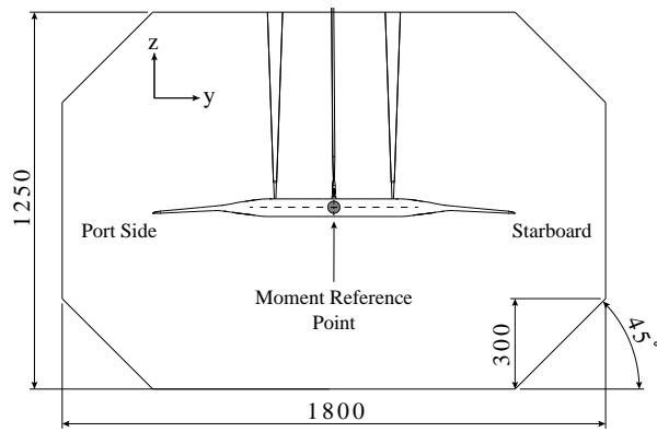
(a) Schematic of the LTT cross-section viewed downstream at \alpha = 0^\circ . Dimensions are given in mm.
