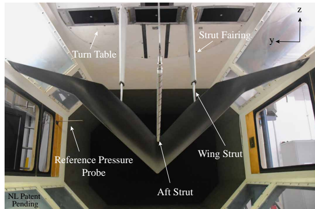
(b) Model setup in the test section, viewed from below and looking upstream at \alpha = 10^\circ .
