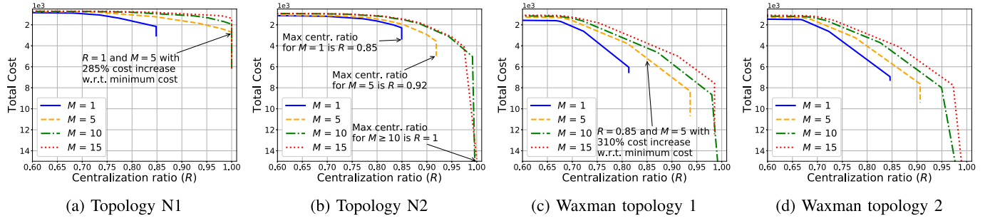
Fig. 7. Pareto Analysis in Low Routing Cost Scenario: Study of the cost J and centralization R in two real and two synthetic networks; with routing cost c_d = 5, \forall p \in \mathcal{P} , and traffic load \lambda_n = 150, \forall n \in \mathcal{N} .
