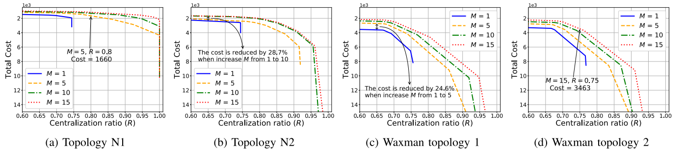
Fig. 9. Pareto Analysis in Low DU Traffic Scenario: Study of the cost J and centralization R in two real and two synthetic networks; with routing cost c_d = 5, \forall p \in \mathcal{P} , and traffic load \lambda_n = 250, \forall n \in \mathcal{N} .
