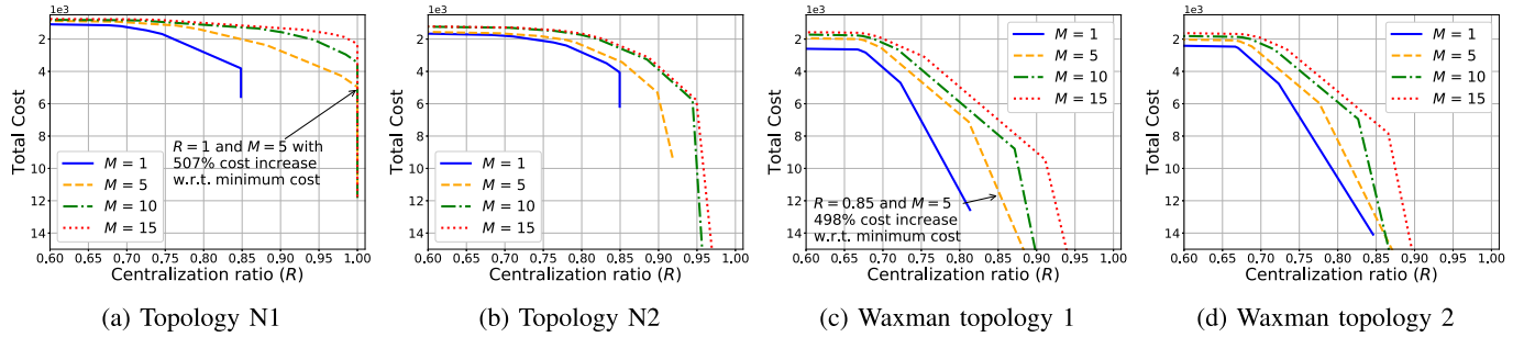
Fig. 8. Pareto Analysis in High Routing Cost Scenario: Study of the cost J and centralization R in two real and two synthetic networks; with routing cost c_d = 10, \forall p \in \mathcal{P} , and traffic load \lambda_n = 150, \forall n \in \mathcal{N} .
