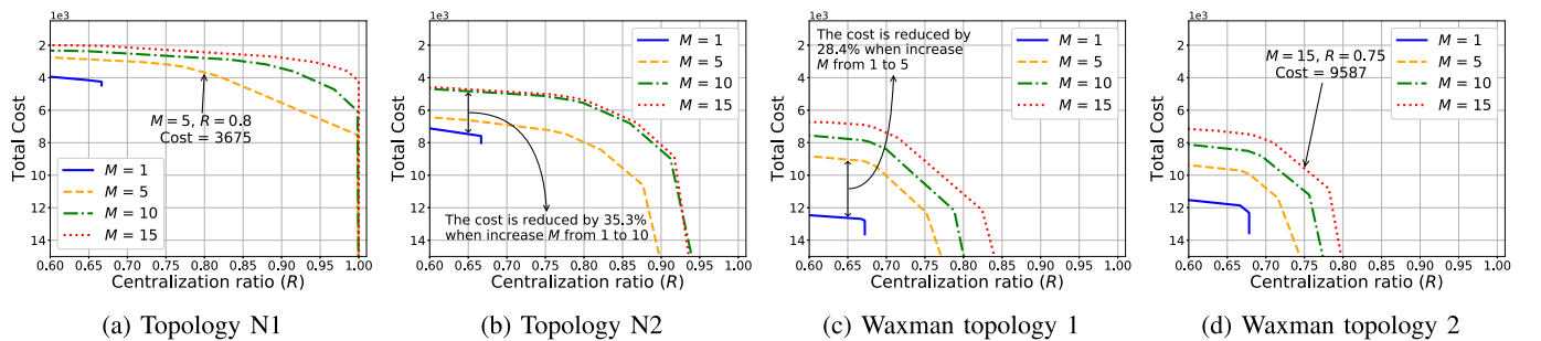
Fig. 10. Pareto Analysis in High DU Traffic Scenario: Study of the cost J and centralization R in two real and two synthetic networks; with routing cost c_d = 5, \forall p \in \mathcal{P} , and traffic load \lambda_n = 500, \forall n \in \mathcal{N} .
