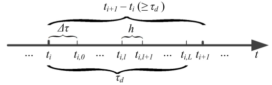
Fig. 3. The time sequence between two consecutive switching instants.
