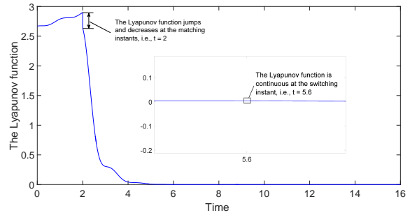
Fig. 6. The proposed Lyapunov functions with a zoomed detail around t = 5.6 .
