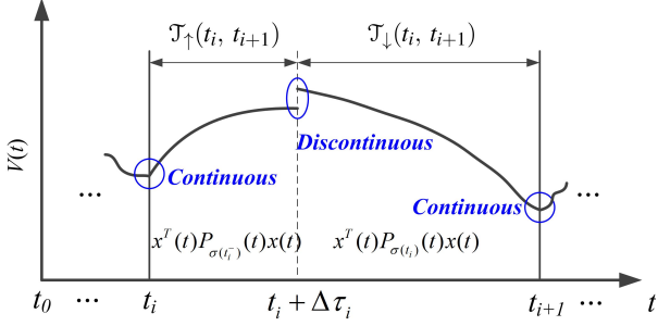
Fig. 2. The proposed Lyapunov function (6).
