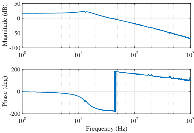
Fig. 6. Frequency response data of plant as seen from actuator ‘1A’ to position of mass ‘3’ attached to same actuator.
