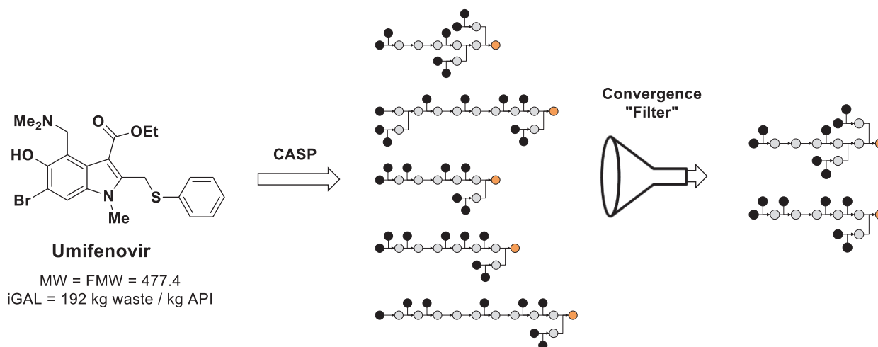
Figure 10. Integrating convergence to CASP applications as an algorithm to filter for more efficient synthesis plans for Umifenovir API.
