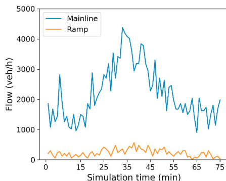
Fig. 6. Demand profile generated for an average scenario under the LQR control case
