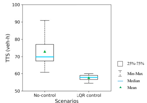
Fig. 4. Comparison of no-control and LQR control scenario
