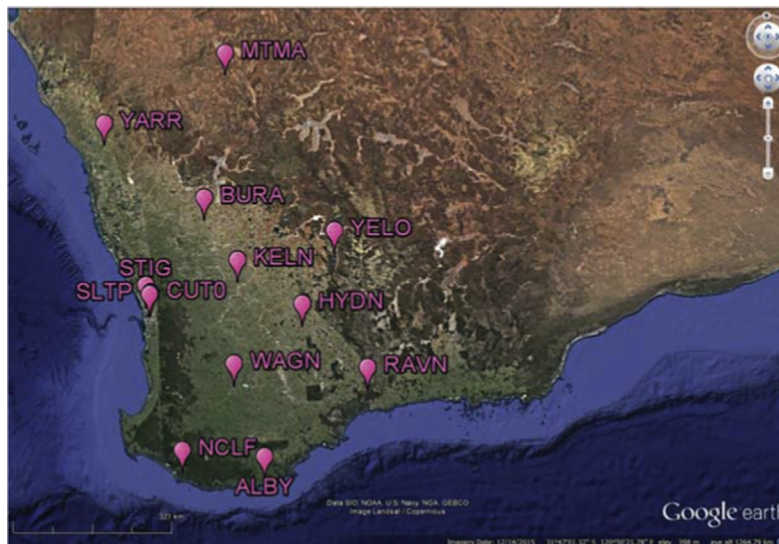
Fig. 4. DF Network B in Western Australia with the largest inter-station distance of around 757 km. Map data: Google, Data SIO, NOAA, U.S. Navy, NGA, GEBCO, Image Landsat/Copernicus (Google Earth, 2015).
