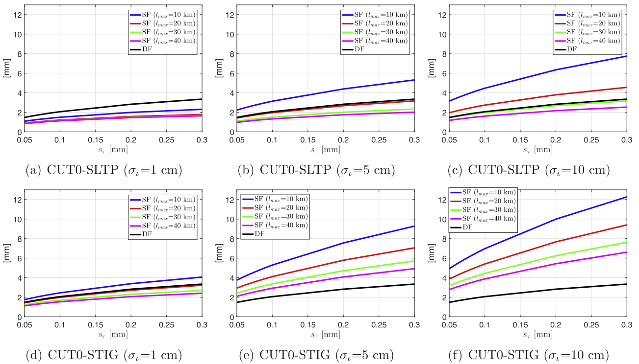
Fig. 8. Average formal standard deviations of the rZWDs for (a, b, c) baseline CUT0-SLTP of around 3 km and (d, e, f) baseline CUT0-STIG of around 17 km. The parameter \sigma_r (Eq. (A.3)) was set to be (a, d) 1 cm, (b, e) 5 cm and (c, f) 10 cm, respectively. Partial ambiguity resolution was enabled with a predefined success rate of 99.9%. For the SF network A and the DF network B, ionosphere-weighted and -float models were applied in the processing, respectively.
