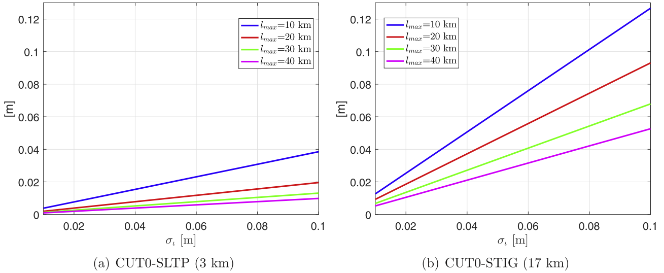
Fig. 7. Standard deviations of the ionospheric spatial constraints (Eq. (A.3)) for (a) baseline CUT0-SLTP of around 3 km and (b) baseline CUT0-STIG of around 17 km. The mean elevation angle \bar{e}^s (Eq. (A.3)) was assumed to be 50 degrees.
