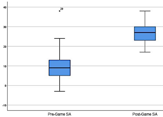
Figure 4.3. Boxplot to identify significant outliers.
