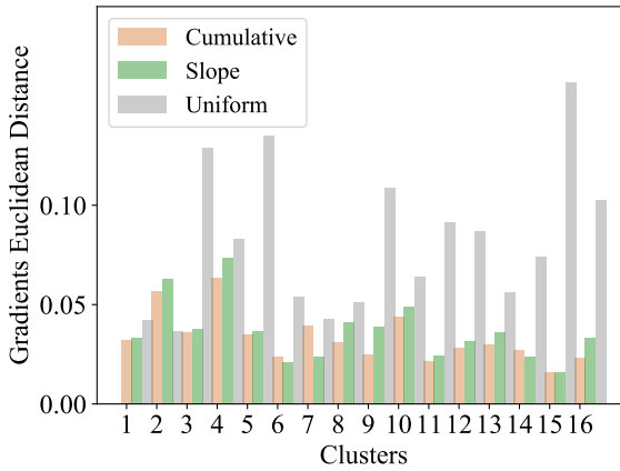
Fig. 3.6: Comparing the Euclidean distance between gradients of the ground truth of truly using all frames to our efficient approximation per cluster for cumulative clustering, slope clustering and uniform grouping on Move4MNIST. Compared to uniform grouping and slope clustering, cumulative clustering results in smaller gradients difference and thus a better approximation.
