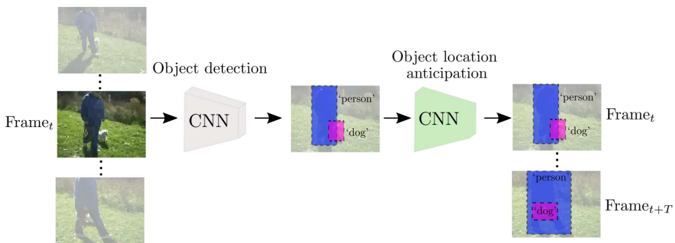
Fig. 1.3: Chapter 2: Efficient video object detection. The proposed video object detection method starts from individual video frames at timestep t and detects the object locations via a convolutional neural network (CNN). Subsequently, the novelty of the method comes from anticipating the future object locations (highlighted in green, here) over the next T frames. Thus, the frames between timestep t and t+T do not need to be processed in the network, leading to efficiency.
