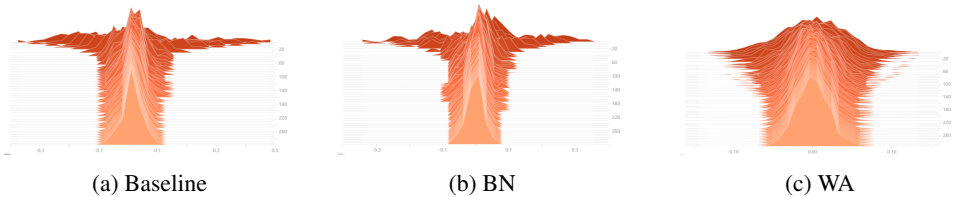
Fig. 5.4: Channel weights distribution of trained ResNet50 versus epoch: (a) channel weights of baseline model. (b) channel weights of BN model. (c) channel weights of WA model. The x-axis represents the value of weights. The y-axis represents the epoch. From top to bottom, the epoch varies from 1 to 300. WA makes the distributions of channel weights symmetric around 0. With a symmetric distribution around zero for the weight, the activation can also have a symmetric distribution around zero.
