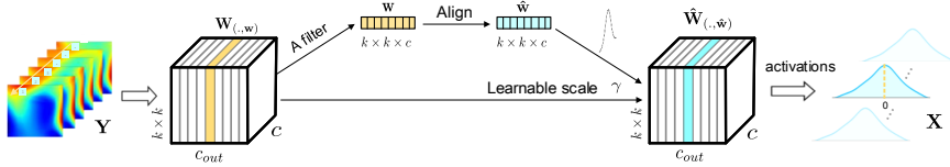
Fig. 5.1: Overview of WeightAlign (WA): Aligning filter weights allows normalizing channel activations. The weight \mathbf{W} of an arbitrary convolutional layer is composed with C_{out} filters with size C \times k \times k . Within a filter (yellow region in the left side), we first flatten it to a vector and then apply our proposed WA in Eq. (eq. (5.10)) to normalize the filter weights with an introduced learnable parameter \gamma . Normalizing weights of each filter in forward pass can realize the normalization of activations within each channel. Details in Section 5.3.
