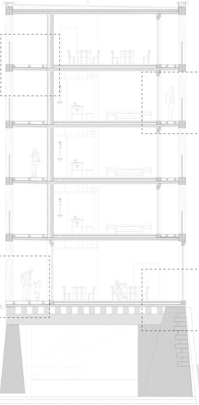
section detail
