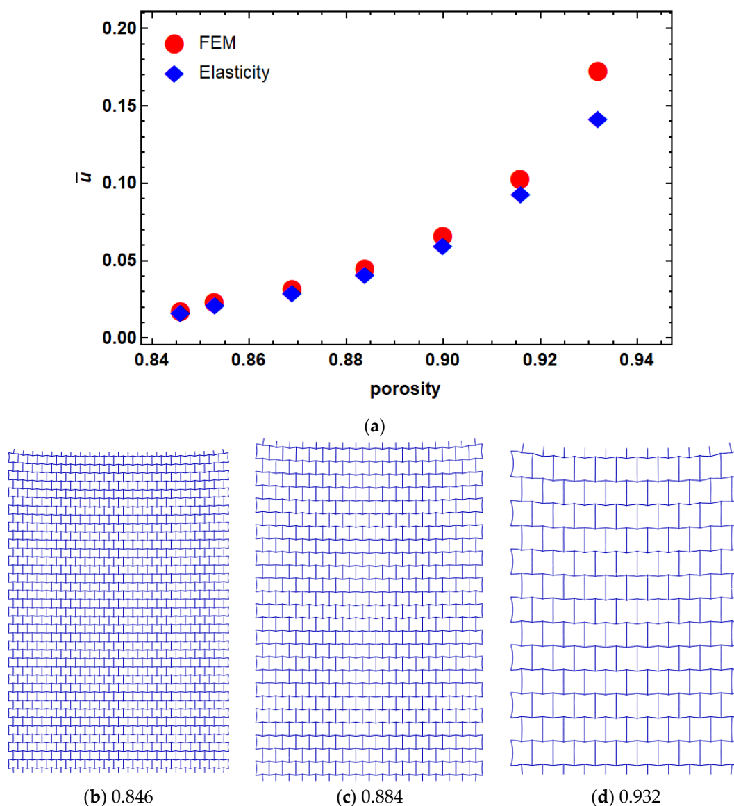
Figure 3. Dimensionless displacement of re-entrant structure with different porosities (a) porosity. Examples of different porosity levels are shown subfigures (b) 0.846, (c) 0.884 and (d) 0.932.
