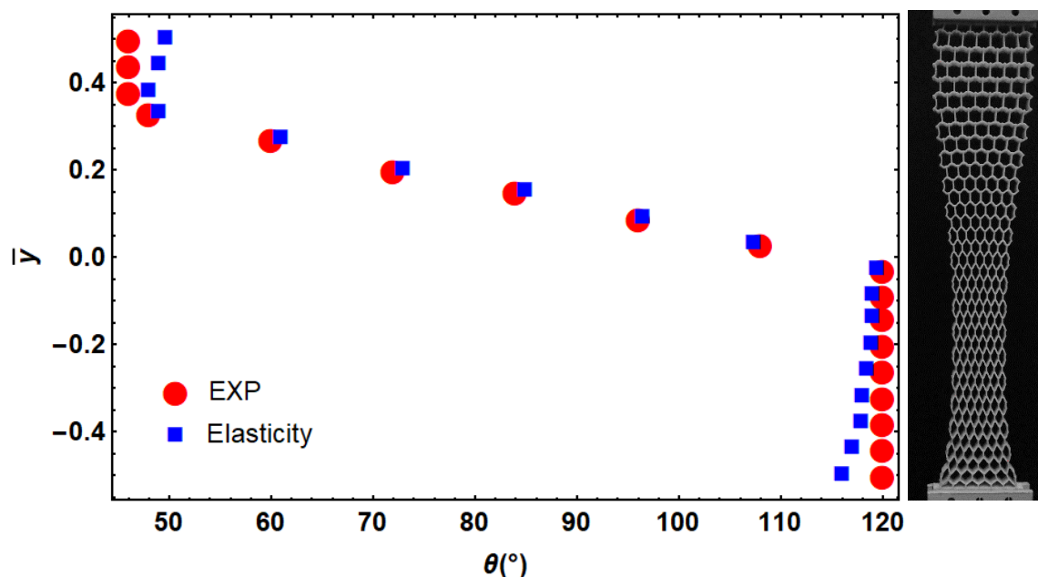
Figure 8. Comparison between the designed angle of cells with the presented approach and those obtained from experimental results presented in [17] for the desired deformation.
