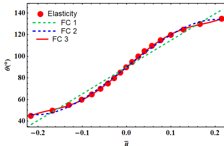
Figure 6. Different fitting curves (FC) used to find the relationship between the unit cell angle vs. the dimensionless lateral displacements using the elasticity theory. The corresponding fitting equations are shown in Table 1.
