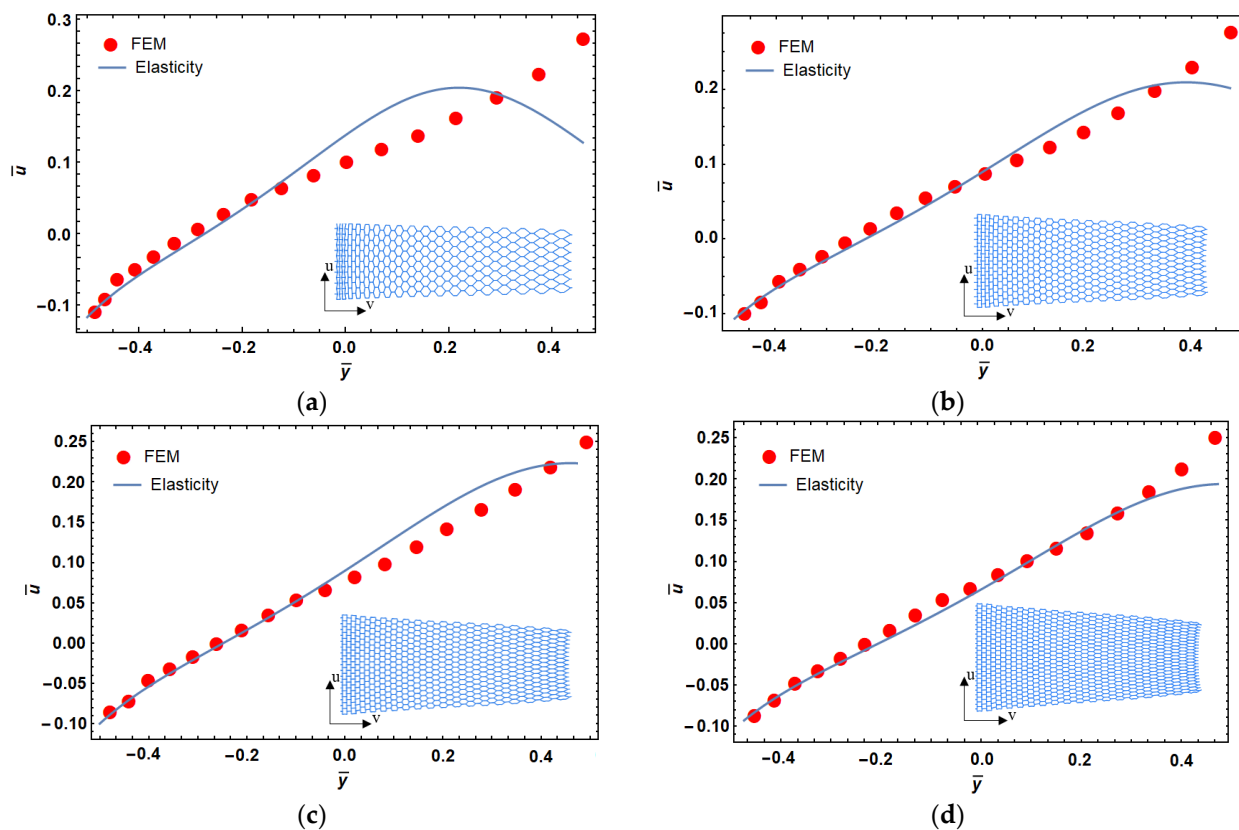
Figure 4. Porosity effect on dimensionless displacement in functionally graded reentrant structure; 94% (a), 92% (b), 90% (c), and 88% (d) porosity.
