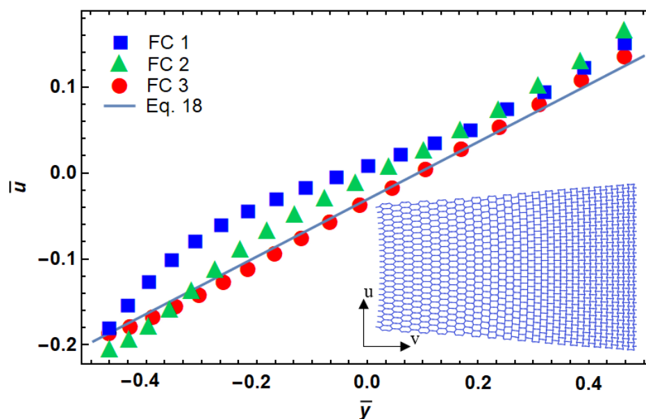
Figure 7. Functionally graded design of a re-entrant cellular plate with non-dimensional lateral and longitudinal deformation.
