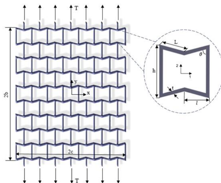
Figure 1. Re-entrant lattice structure is made of hexgonal unit cells whose geometrical parameters are shown in the subfigure. The lattice structure is supposed to be under uniaxial tensile loading.
