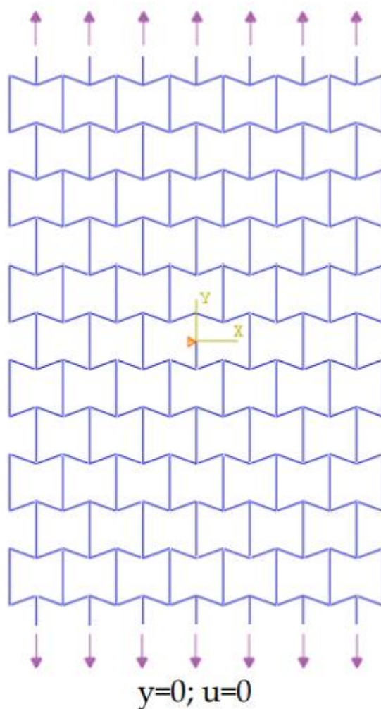
Figure 2. Finite element model and boundary conditions.
