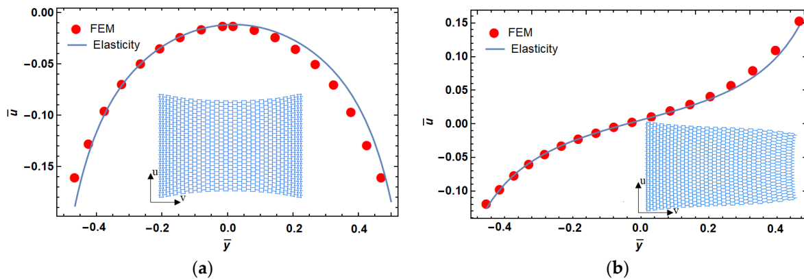
Figure 5. Dimensionless displacement in functionally graded re-entrant structure for the desired parabola (a) and cubic (b) shapes.
