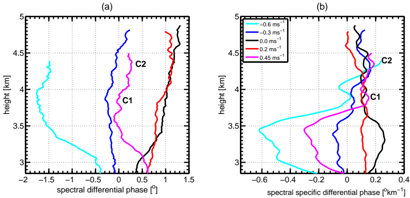
Figure 4.6: shows height profiles for fixed Doppler velocity bins, -0.6 \text{ ms}^{-1} (light blue), -0.3 \text{ ms}^{-1} (dark blue), 0.0 \text{ ms}^{-1} (black), +0.2 \text{ ms}^{-1} (red), and +0.45 \text{ ms}^{-1} (magenta), for the spectrograms presented in Figure 4.4. (a) shows the \Phi_{DP} -profiles and (b) the K_{DP} -profiles for the constant Doppler velocities. C1-C3 are markers that refer to the ones of Figure 4.4 and discussed in the text.
