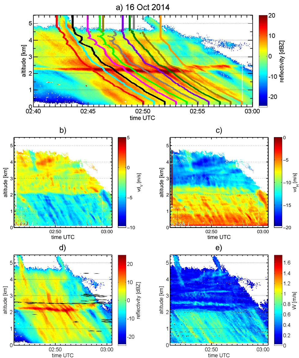
Figure 2.8: Overview of a raining cloud case of ACCEPT observed 16 th October 2014, 0240 - 0300 UTC. a) shows the reflectivity overlaid with 10 retrieved fall streaks separated by one minute time difference from 0250 to 0259 UTC. b) and c) show plots of the vertical and horizontal Doppler velocities, respectively. d) is the reflectivity overlaid with the retrieved supercooled liquid water signatures from lidar (black) [19]. The Doppler spectrum width is shown in e).
