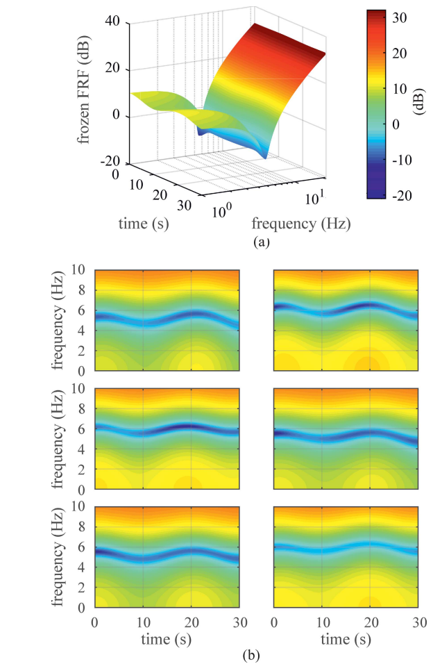
Fig. 8. Results obtained using the kernel-based method. (a) Estimated frozen FRF, using kernel-based regression. (b) Frozen FRF for all trials recorded in a single participant in the condition where voluntary torque was sinusoidally varied between 5% and 20% of maximum voluntary torque. Color scale same as in (a).
