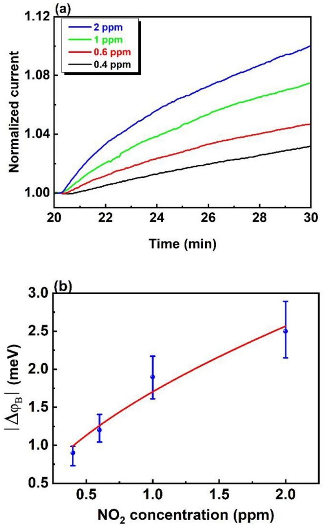
Figure 6. (a) Magnification of the signal recorded during the exposure at different concentrations of NO 2 . The signals are normalized at the values I_0 prior to the gas inlet. (b) Absolute value of SBH vs NO 2 concentration as calculated from panel (a).
