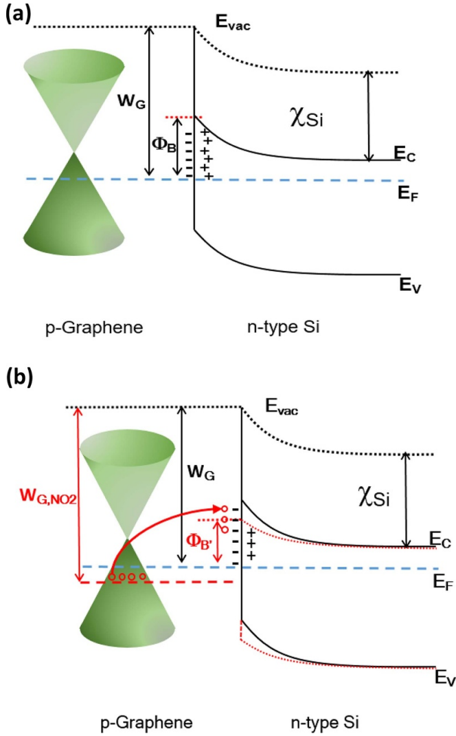
Figure 5. Band diagram of the heterojunction (a) before and (b) after the exposure to NO 2 . For the sake of clarity, the band structure of graphene was designed similar as that of a single layer of graphene. E_{vac} , E_C , E_V and E_F indicate vacuum energy, conduction band, valence band and Fermi level of the n-type Si, respectively.
