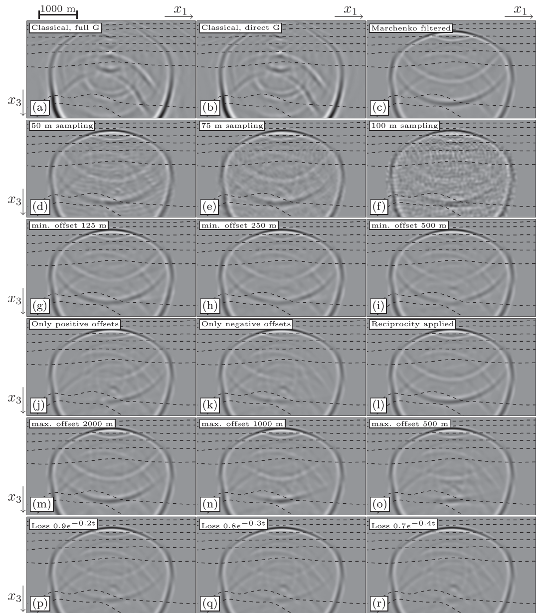
Figure 7. Snapshots of the homogeneous Green's function at t = 400 ms, retrieved using varying limitations of the reflection response, following the workflow in Figure 5a. All wavefields have been convolved with a 15 Hz Ricker wavelet. (a) Result from Figure 6f, (b) result from Figures 6i, and (c) result from Figure 6o, the latter used as a benchmark for the other results. (second row) Homogeneous Green's function obtained, when the reflection response has a source and receiver spacing of (d) 50, (e) 75, and (f) 100 m. (third row) Homogeneous Green's function obtained when the reflection response is missing the small source-receiver offsets up to a distance of (g) 125, (h) 250, and (i) 500 m. (fourth row) Homogeneous Green's function obtained when the reflection response contains (j) only positive source-receiver offsets, (k) only negative source-receiver offsets, and (l) has all source-receiver offsets restored using source-receiver reciprocity. (fifth row) Homogeneous Green's function obtained when the reflection response has an aperture limited to (m) 2,000, (n) 1,000, and (o) 500 m. (sixth row) Homogeneous Green's function obtained when the reflection response has a loss applied to it of (p) 0.9e^{-0.2t} , (q) 0.8e^{-0.3t} , and (r) 0.7e^{-0.4t} .
