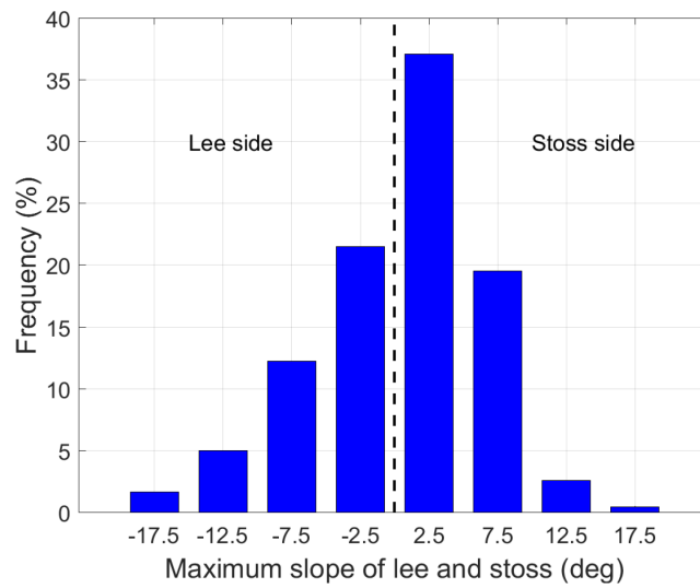
Figure 17. Histogram of maximum slopes computed in 32 typical areas with megarripple structures.
