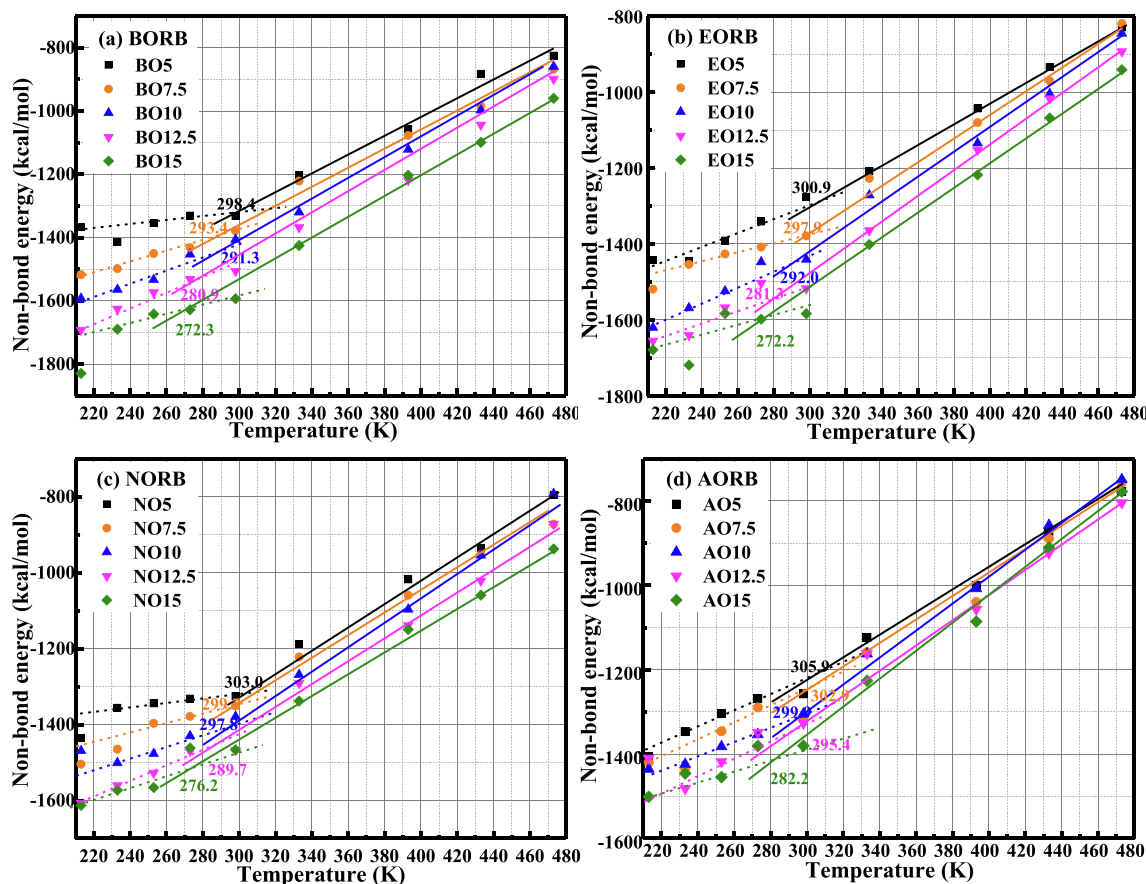
Fig. 16. The E_N -T curves of rejuvenated bitumen.
