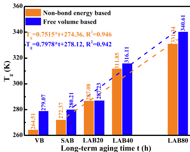
Fig. 17. The glass transition temperature T_g values of virgin and aged bitumen.
