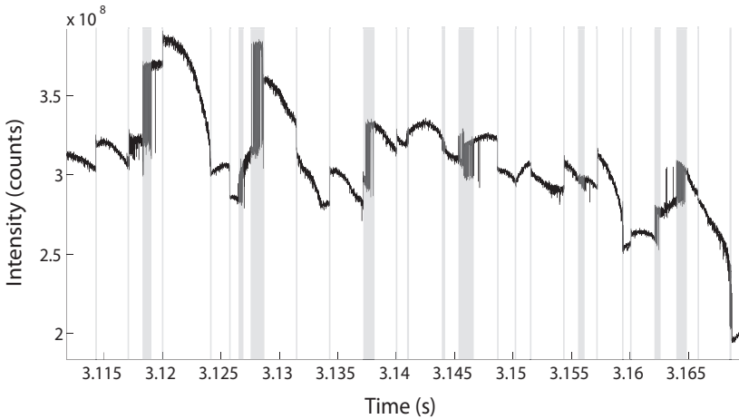
Figure 4.9: Mode zones (white) and mode-hop zones (gray) produced by the tuning of the wavenumber using an external cavity.
