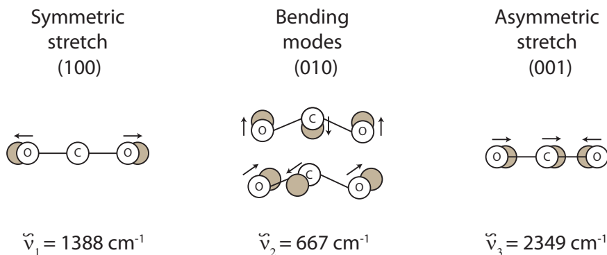
Figure 2.3: Vibrational modes of carbon dioxide.
