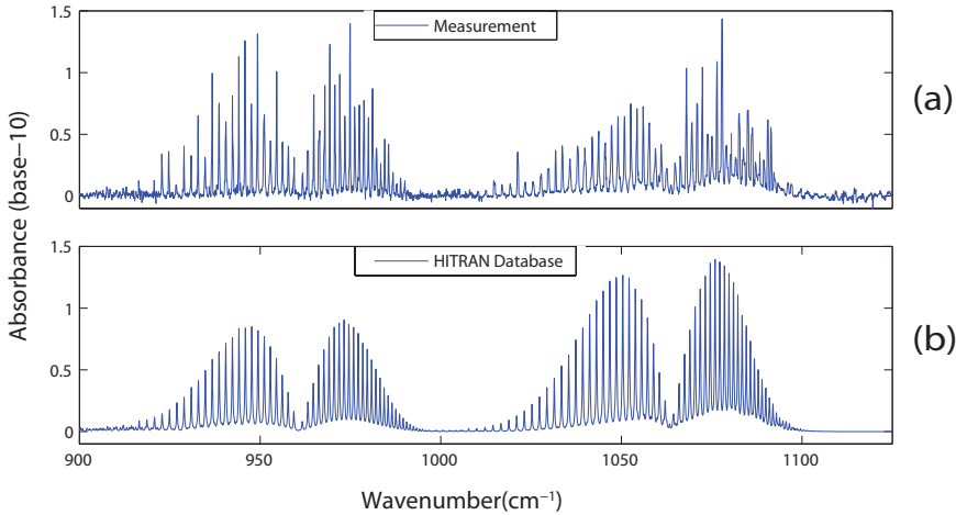
Figure 3.16: Spectrum of 15% of CO 2 in an atmosphere of N 2 at 500 mbar. (a) Experimental measurement. (b) HITRAN database.
