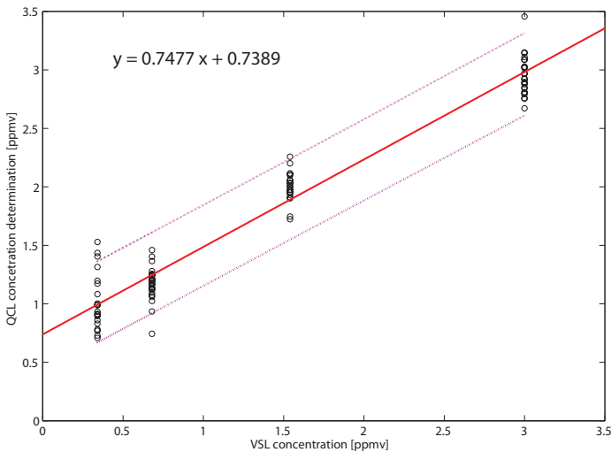
Figure 5.3: Calibration curve of the QCL spectrometer using acetone mixtures provided by the Dutch Metrology Institute. The equation corresponds to the linear fit of the calibration.
