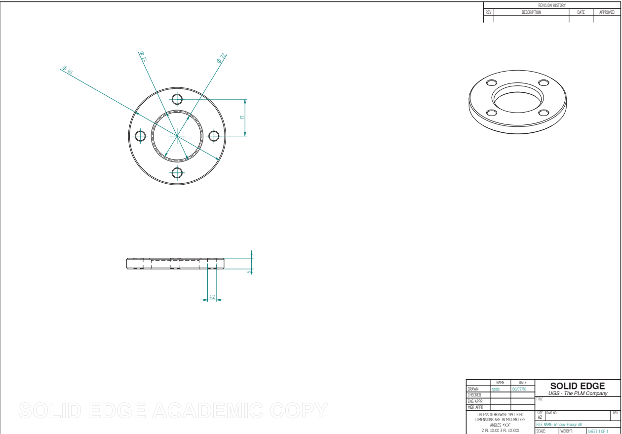
Figure A.16: Flange holding the ZnSe input window.
