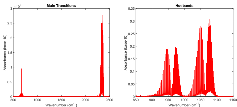
Figure 2.6: Absorption spectrum of the main transitions and hot bands of CO 2 . Information from HITRAN database.
