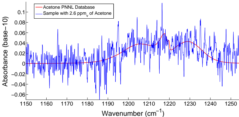
Figure 4.27: Absorbance spectrum of a gas sample with 2.6 ppm v of acetone.
