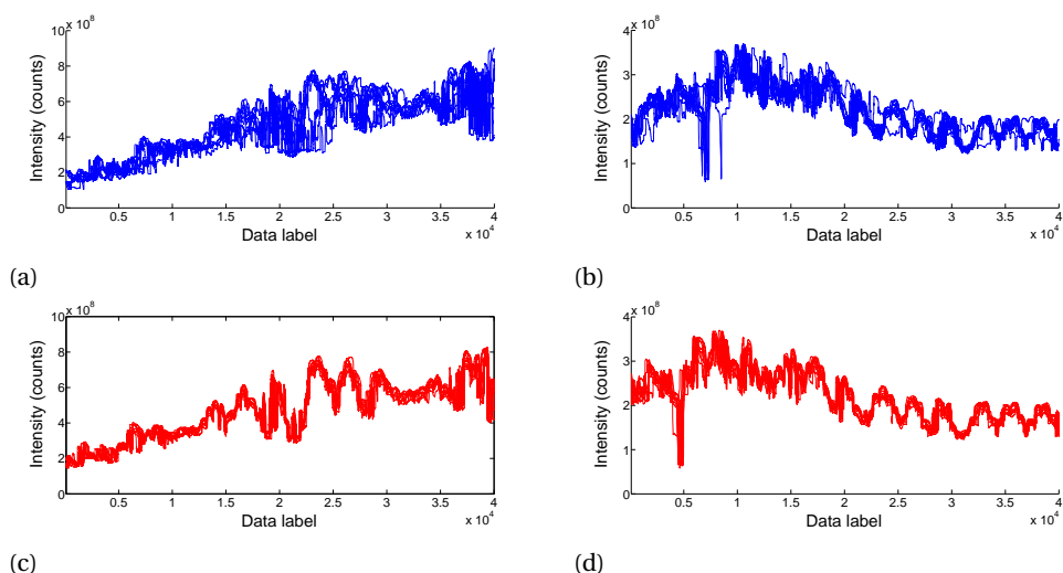
Figure 4.21: Correction using the STW method. (a) Uncorrected normalization signals. (b) Uncorrected main signals. (c) Corrected normalization signals. (d) Corrected main signals.
