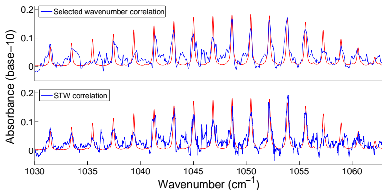
Figure 4.26: Wavenumber calibration of the absorbance spectrum obtained with the scan correlation using selected wavenumbers (upper subfigure) and the STW method (lower subfigure). The red plots show the CO 2 absorbance from the HITRAN database.
