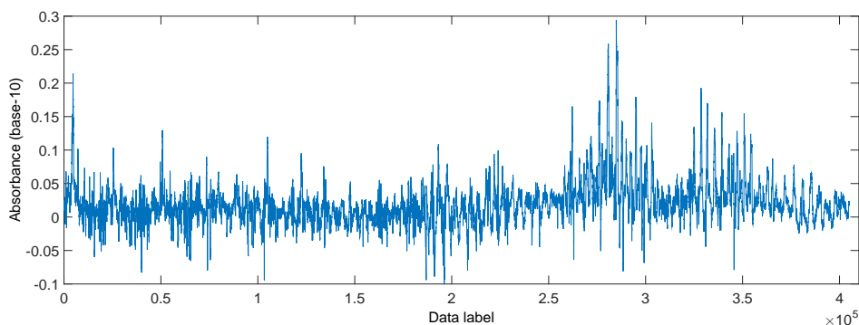
Figure 4.22: Absorbance spectrum of a breath sample in the wavenumber region between 1010 \text{ cm}^{-1} and 1250 \text{ cm}^{-1} obtained using the STW method. the horizontal axis is not calibrated to the corresponding wavenumbers.
