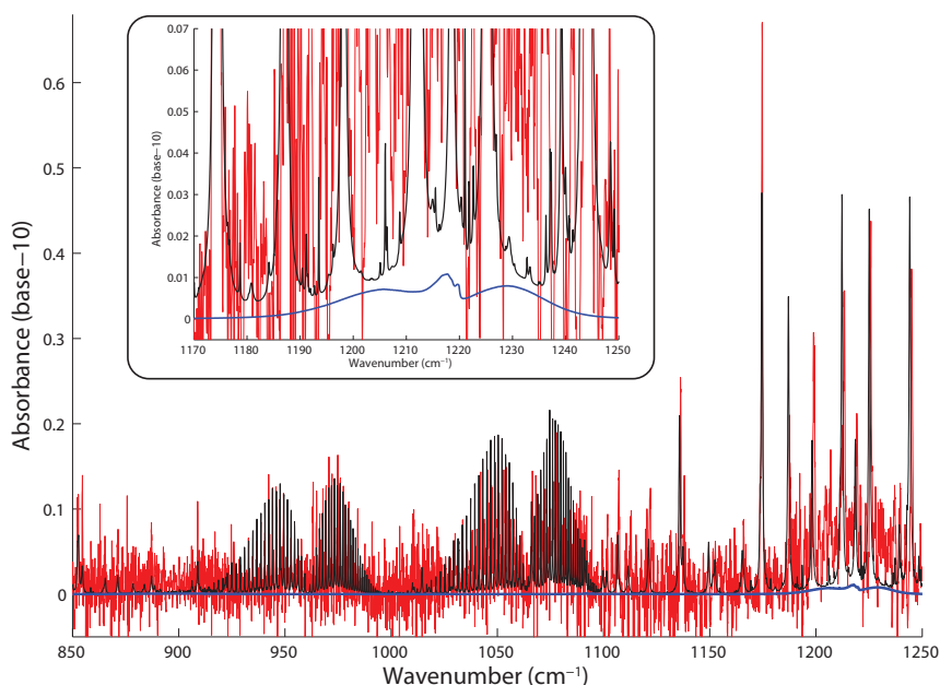
Figure 3.18: Breath sample at 900 mbar and flowing at 500 ml n /min. In black is depicted the theoretical spectrum with 3% of CO 2 and 2% of water from HITRAN database and 500 ppb v of acetone from the PNNL database. In blue is the spectrum of acetone with a concentration of 500 ppb v taken from PNNL database.
