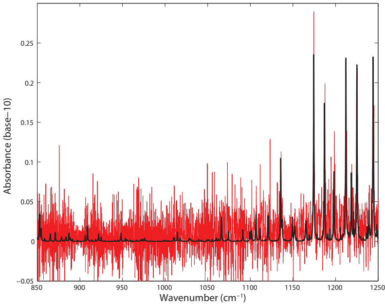
Figure 3.17: Lab air sample at 1001.0 mbar, at a temperature of 23.0 °C and a relative humidity of 31.0%. In black is depicted the spectrum of water from HITRAN database with a concentration of 1 %.
