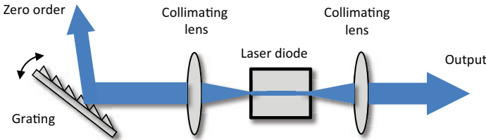
Figure 3.4: Littrow configuration with back extraction. Reproduced with permission from reference 88.
