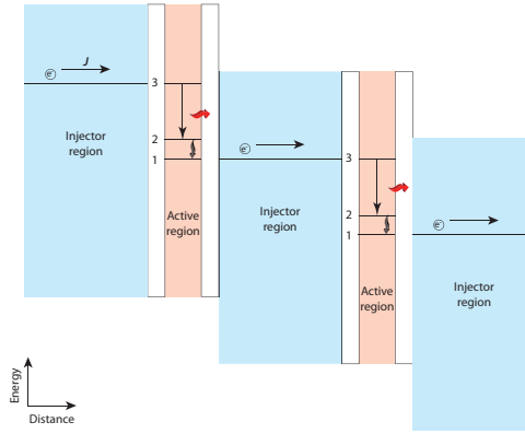
Figure 3.3: Cascade effect. The electrons move along the QCL superlattice, emitting laser light in each active region. The ground level of an active region and the upper state of the next active region are aligned by the injector regions. The alignment of the energy levels is caused by an applied electric field.
