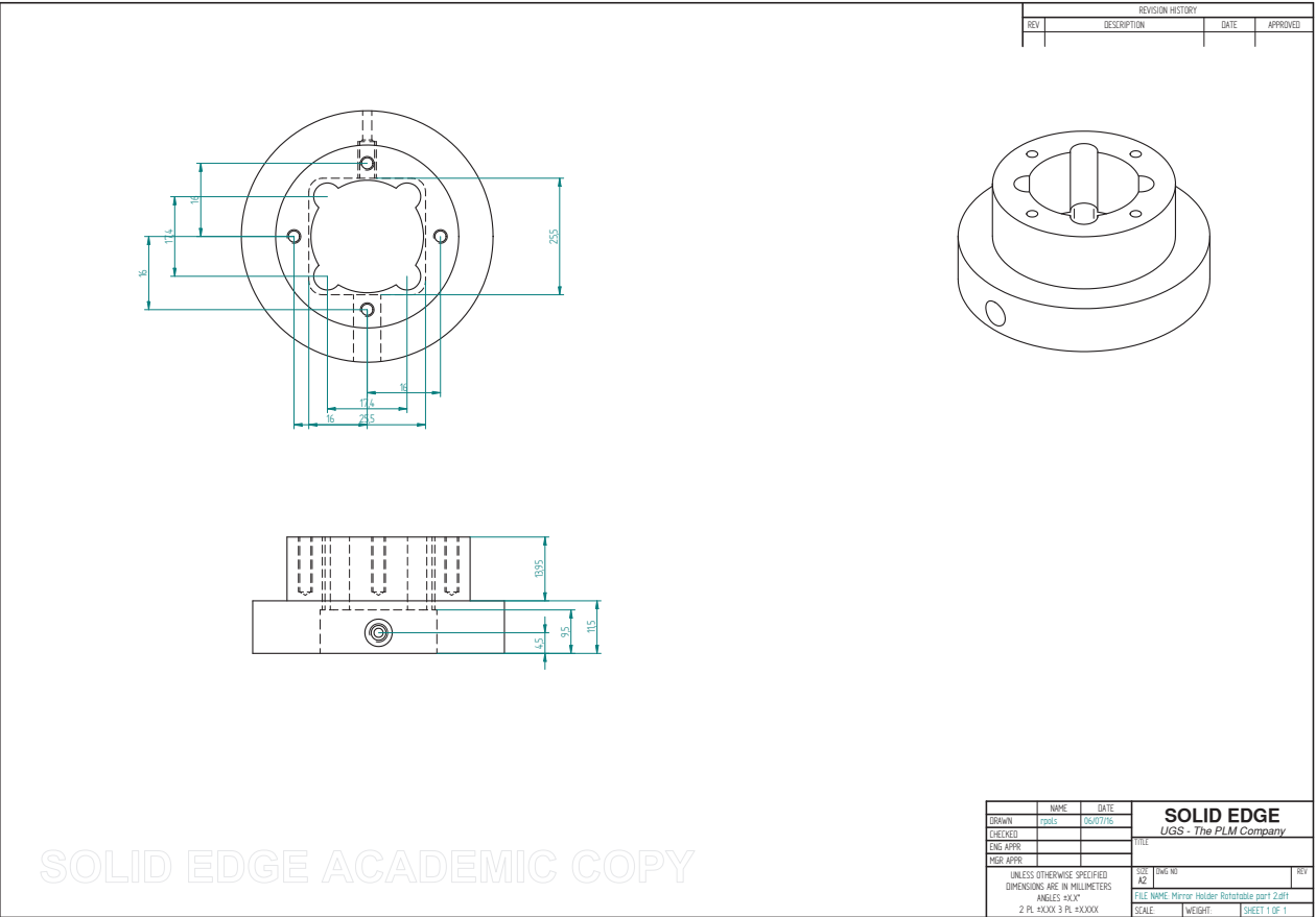
Figure A.12: Details of the support that holds the Newport platform in the rotational mount.
