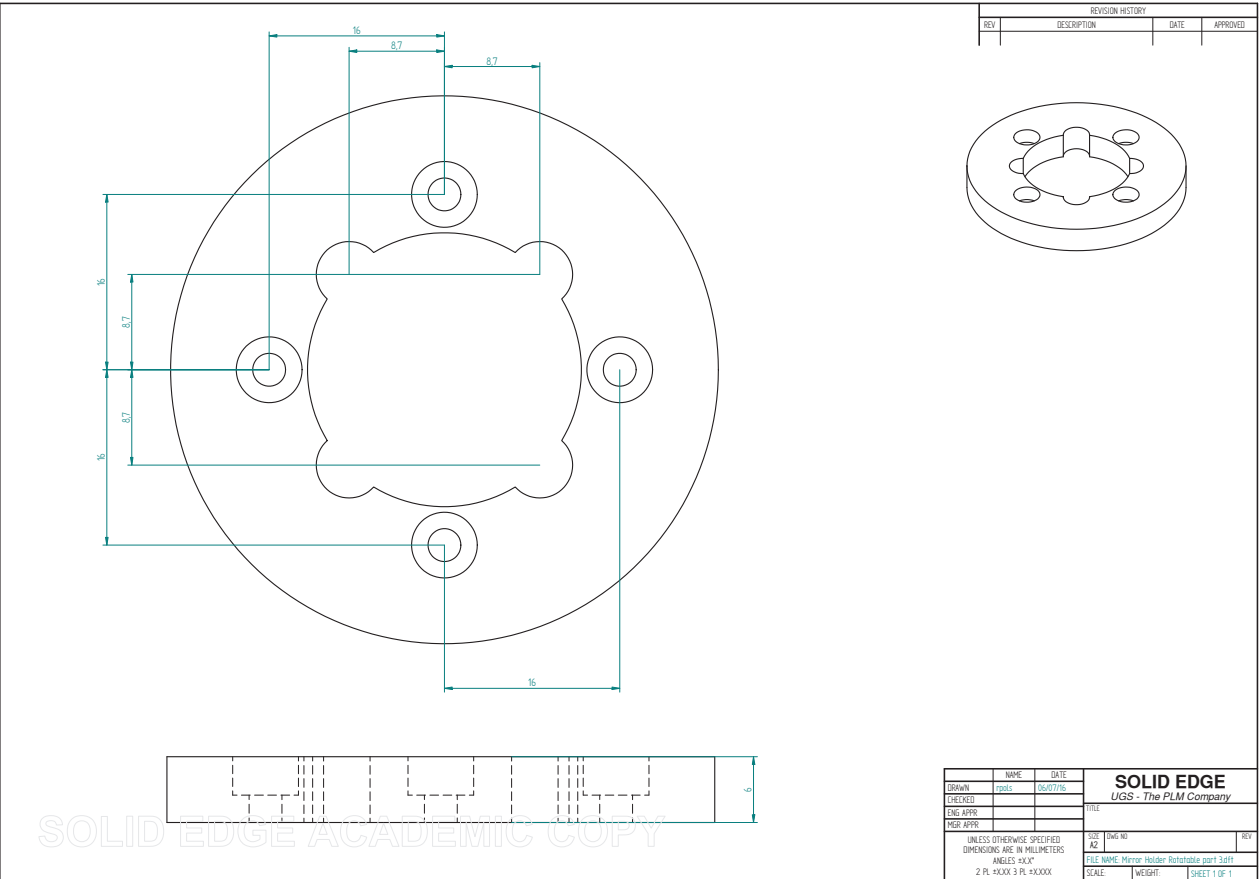
Figure A.1.3: Details of the lock of the rotational mount.
