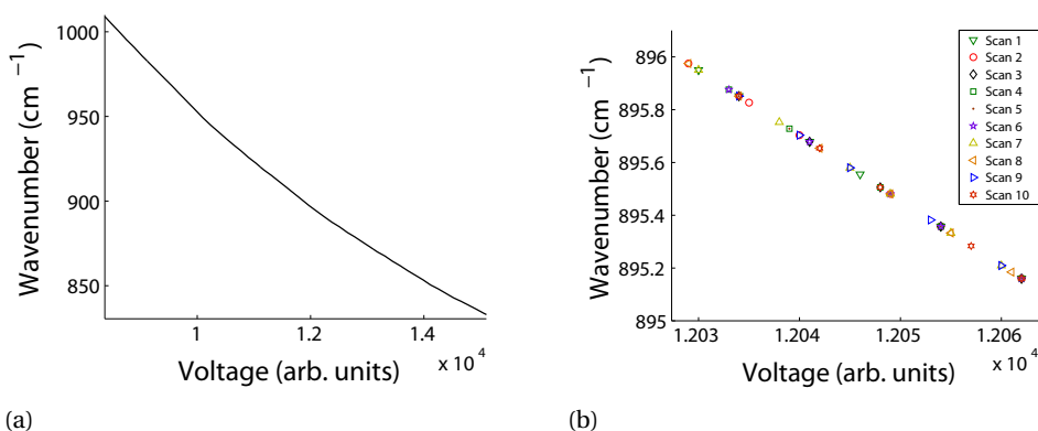
Figure 4.11: Wavenumber dependence on the voltage applied to the piezo scanner.
