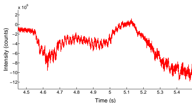
Figure 4.4: Background of the normalization signal. The change in level is clear over a long time range.
