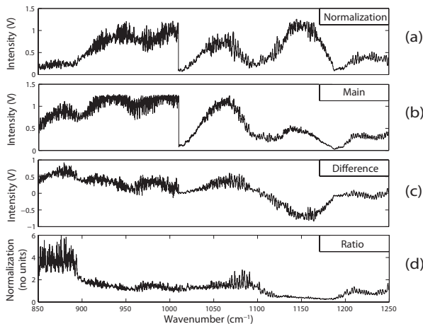
Figure 3.14: The QCL spectrum is measured with two different detectors. In (a) the normalization detector is used while in (b) and the main detector takes into account the effects introduced by the multipass cell. Subfigure (c) shows the difference between the two signals which make explicit the influence of the multipass cell. In subfigure (d) the ratio between the main signal over the normalization signal is presented, this signal should not depend on intensity variations in the QCL emission.
