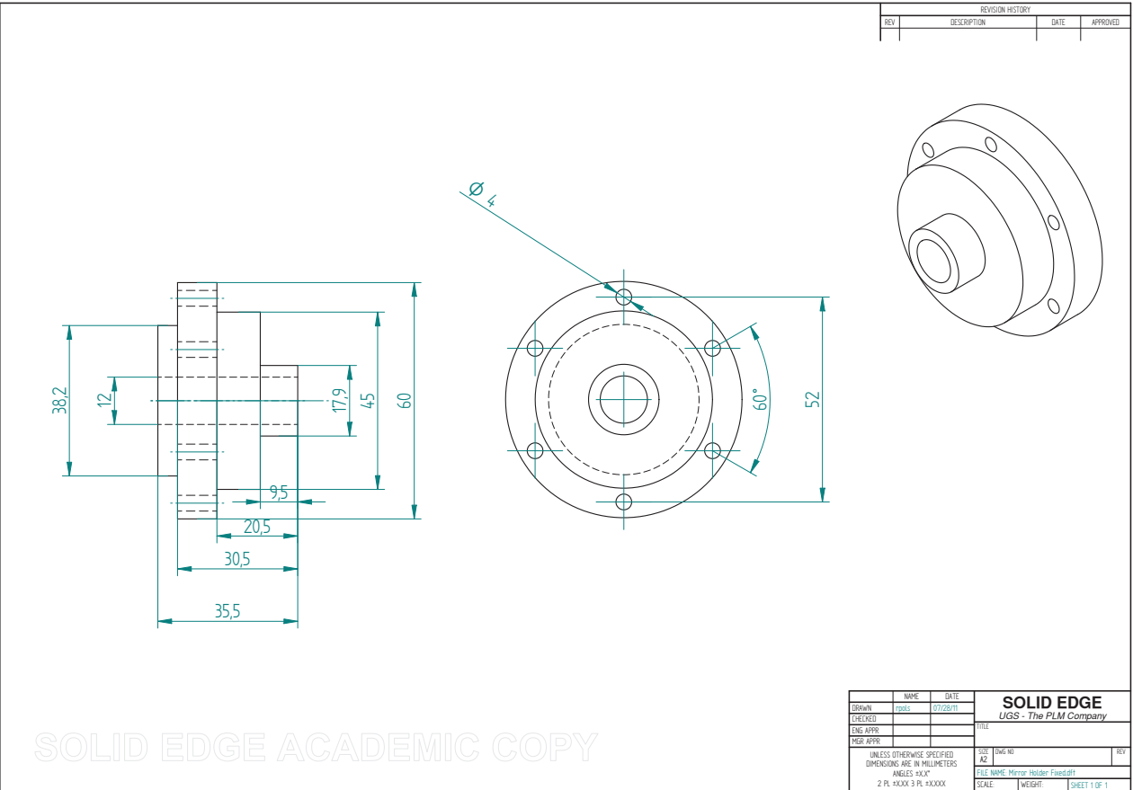
Figure A.8: Details of the support of the mirror.
