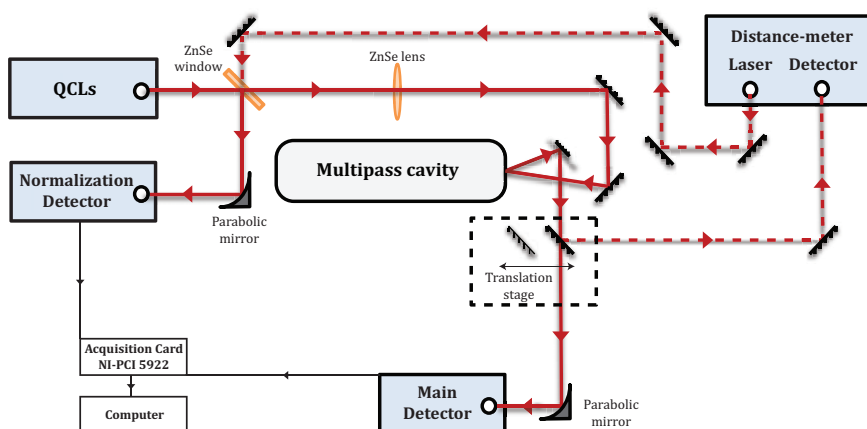
Figure 3.1: Schematic overview of the experimental setup. The translation stage allows to switch between the multipass cell length determination and the measurement configurations.
