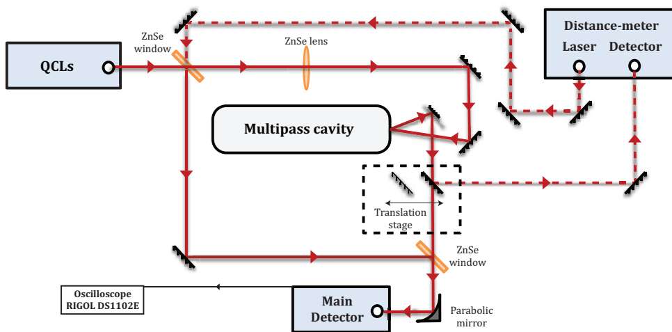
Figure 3.11: Modified experimental configuration to study the robustness of the multipass cell. A ZnSe window is used to send the normalization signal and the signal from the multipass cell into the same detector.
