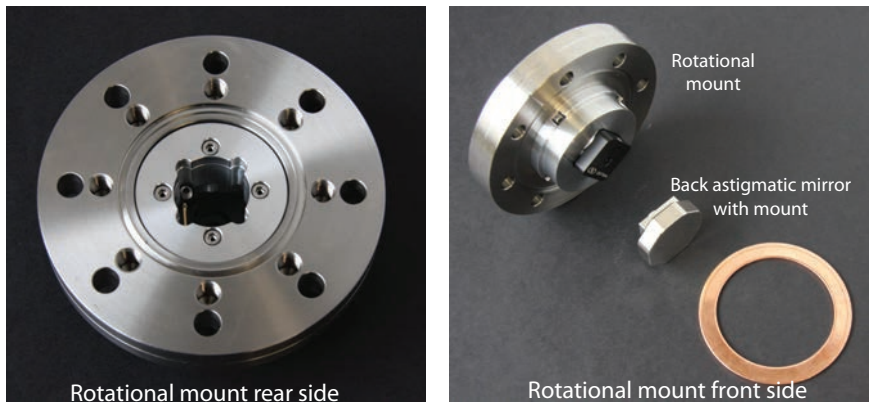
Figure A.10: Picture of the input mirror holder.
