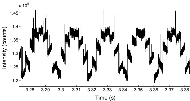
Figure 4.15: Intensity profile of a QCL stabilization region. The temporal width of the mode zones is constant at 2.8616 ms.
