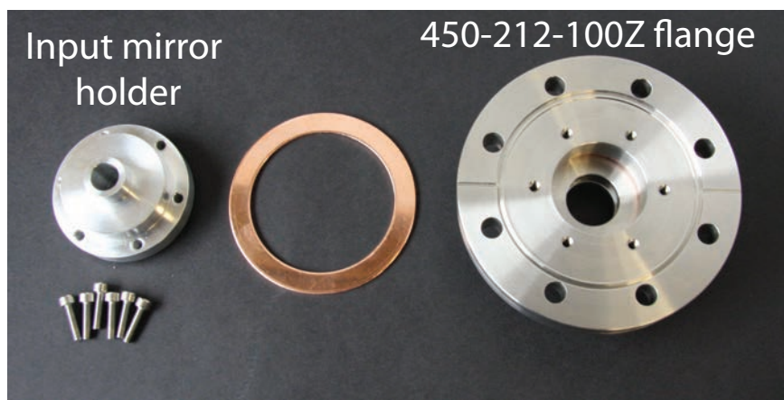
Figure A.6: Picture of the input mirror holder.
