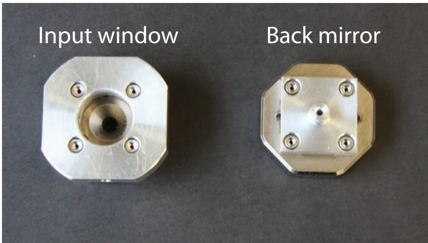
Figure A.3: Mirrors support attached to the rear of the astigmatic mirrors.
