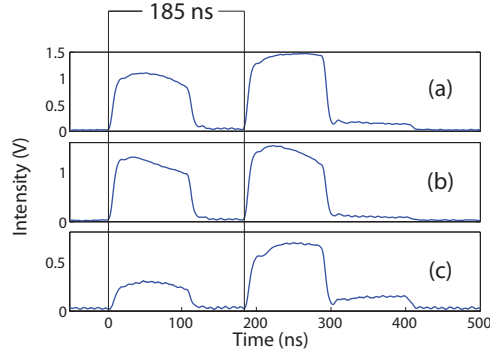
Figure 3.12: Delay time between the normalization and the main signals for three different wavenumbers. (a) 950\text{ cm}^{-1} , (b) 1000\text{ cm}^{-1} and (c) 1150\text{ cm}^{-1} .
