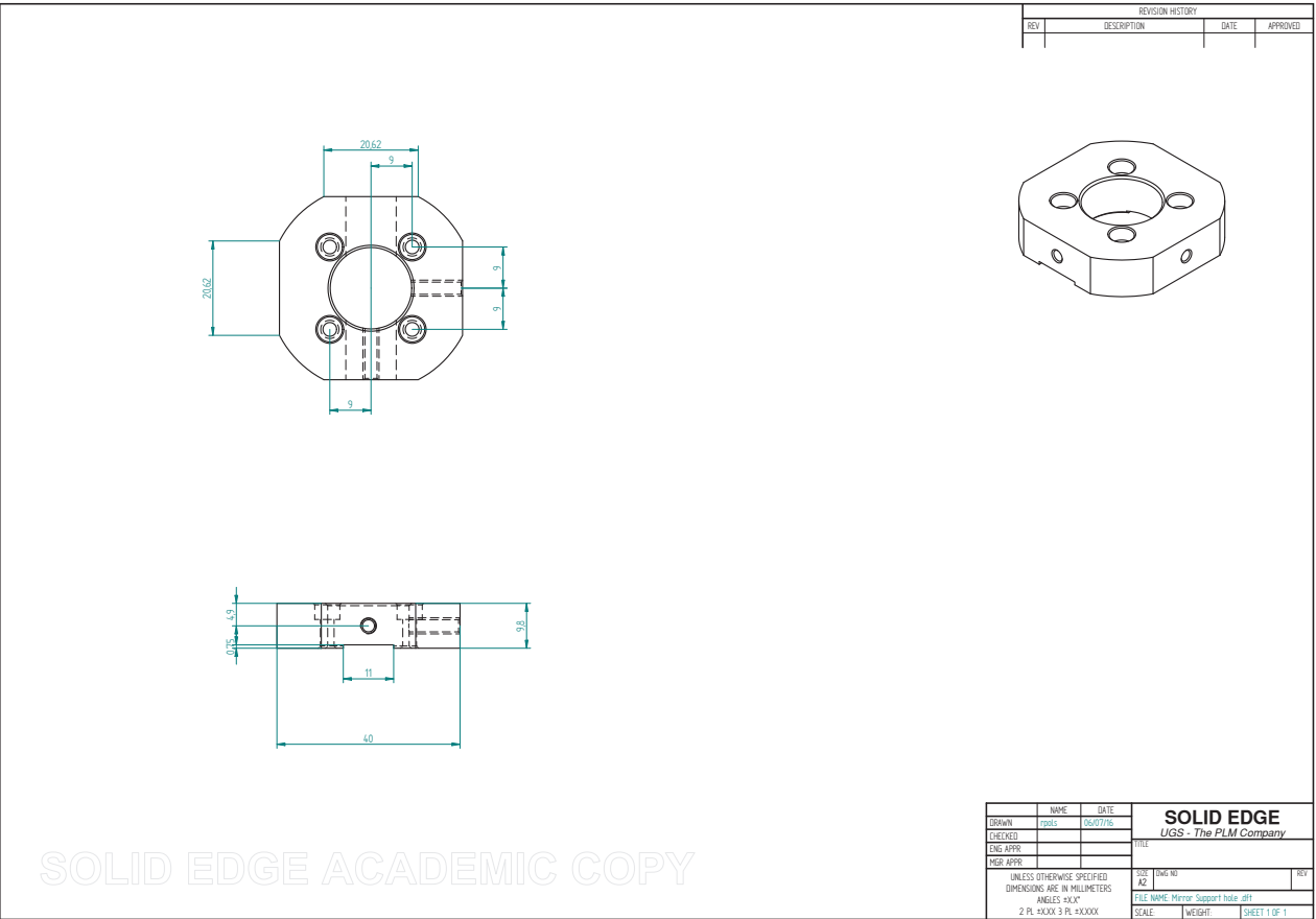
Figure A.4: Details of the support of the mirror.
