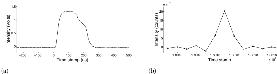
Figure 4.2: QCL pulse digitized using (a) a RIGOL oscilloscope with an acquisition rate of 1 GSa/s and (b) a NI-PCI 5922 acquisition card with an acquisition rate of 10 MSa/s
