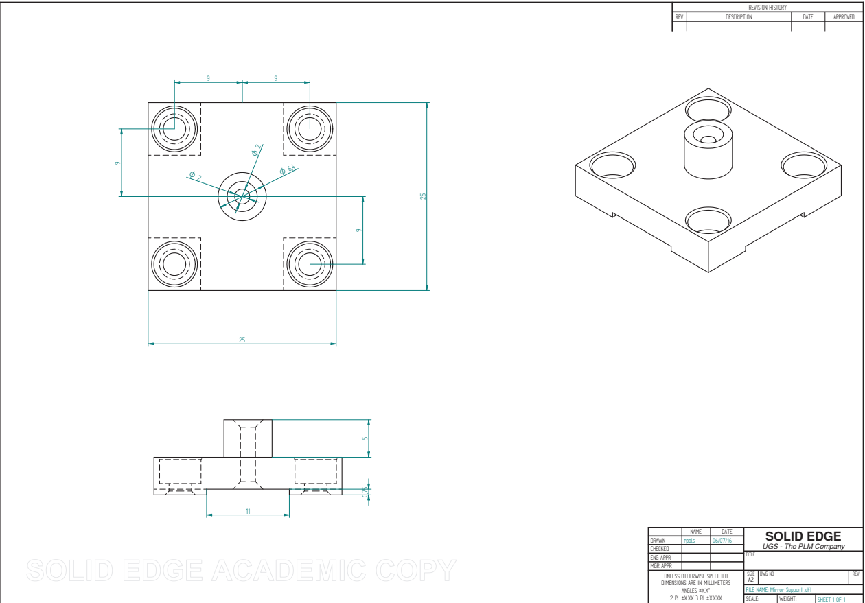
Figure A.5: Details of the support of the mirror.
