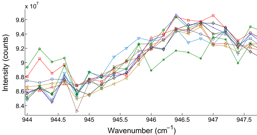
Figure 4.13: Intensity profiles obtained with the LaserScope method.
