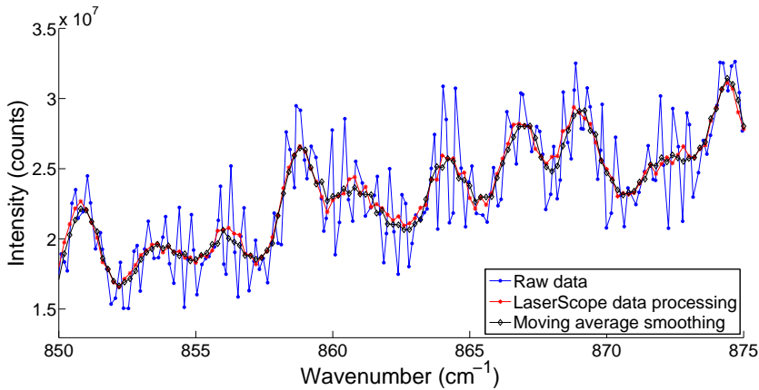
Figure 4.12: LaserScope method. Blue dots correspond to the raw intensity profile, in red is shown the result of the data processing and the black markers are the result of a moving average smoothing and the interpolation applied to the raw data.
