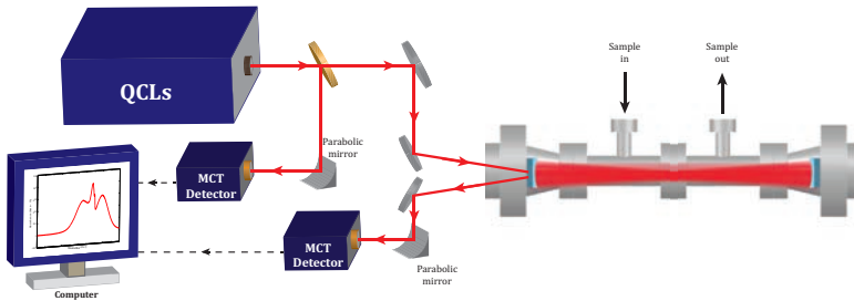
Figure 5.1: Schematic of the experimental setup. Red lines correspond to the laser beam path, solid black arrows show the sample flow and the dashed lines indicate electrical connections.
