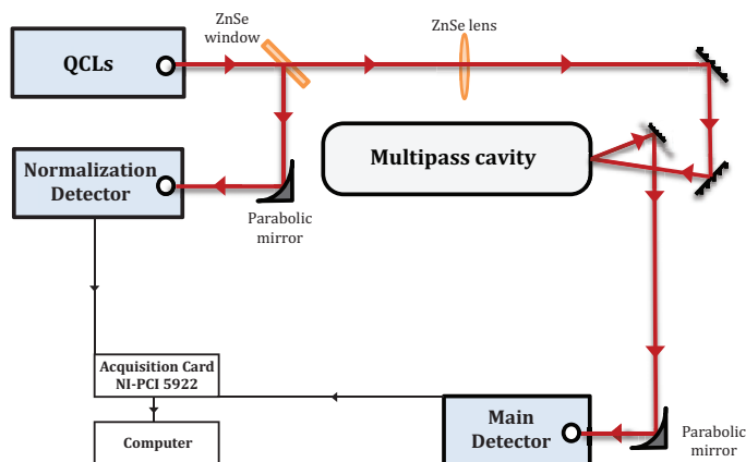
Figure 4.1: Experimental setup scheme. Only the main components of the setup are presented.
