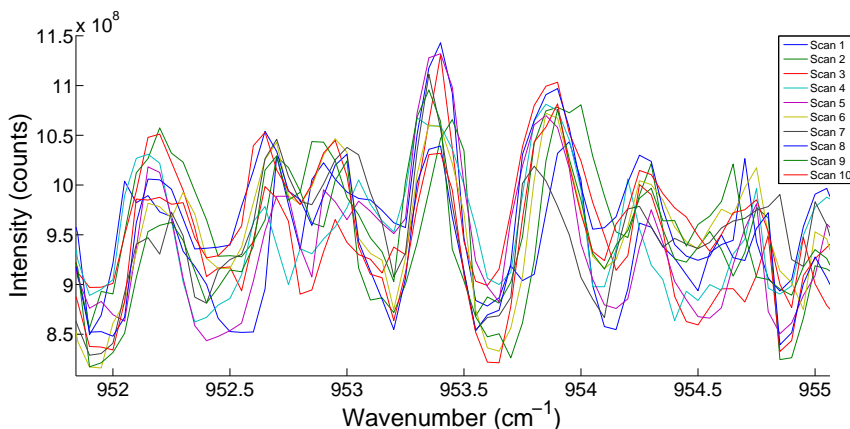
Figure 4.16: Intensity profiles obtained with selected wavenumbers separated by 0.05 \text{ cm}^{-1} . Data obtained with the normalization detector.
