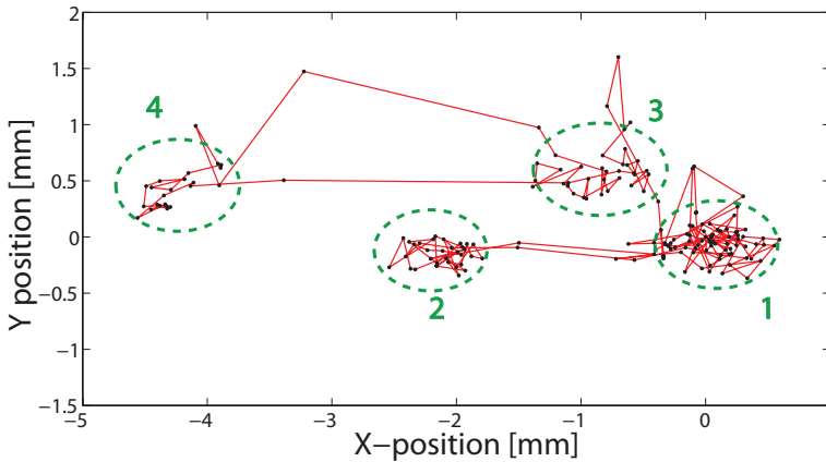
Figure 3.5: Central position of the laser beam over a full wavenumber scan. Reproduced with permission from reference 89.
