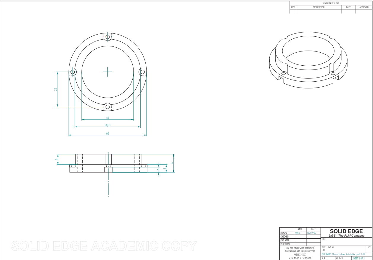
Figure A.11 : Details of the reducer of the rotational mount.
