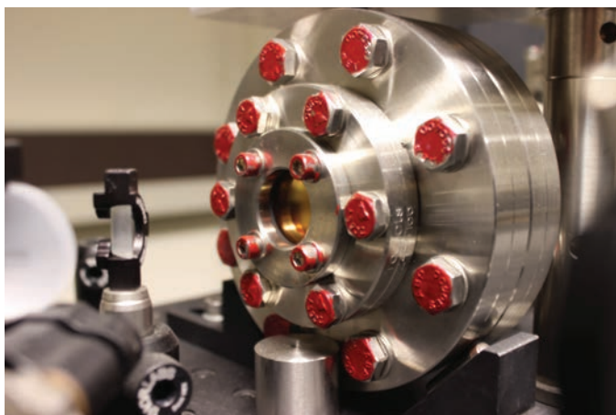
Figure A.15: ZnSe input window mounted in the multipass cell.
