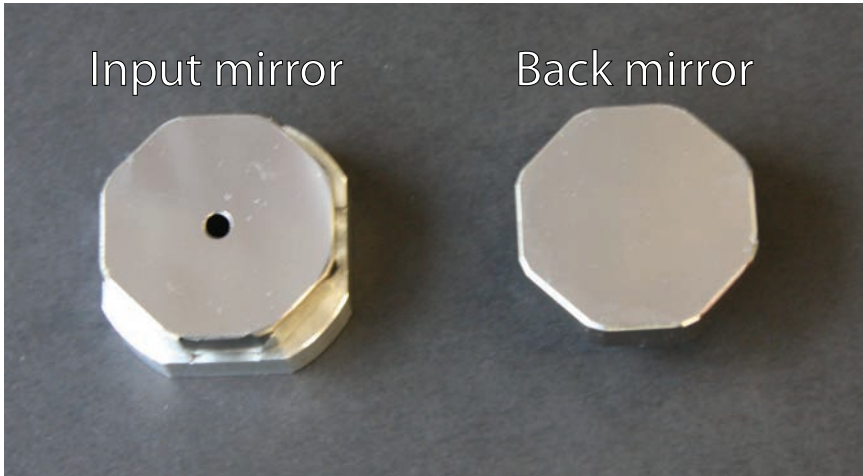
Figure A.2: Astigmatic mirrors.
