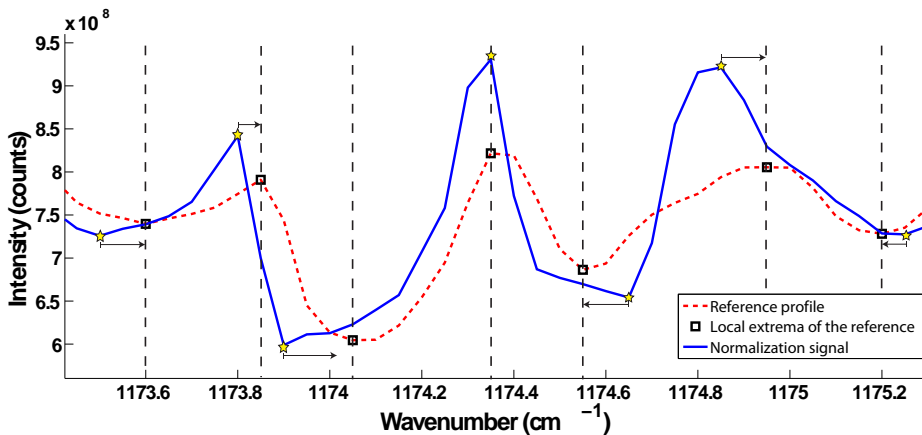
Figure 4.17: Wavenumber correction using the average of the normalization signals as base.
