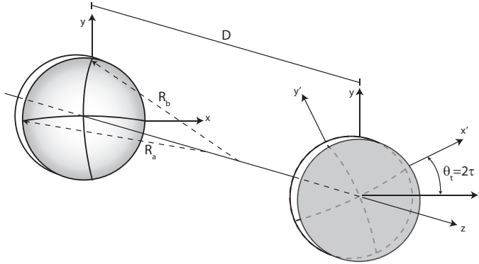
Figure 3.9: Multipass cell with two astigmatic mirrors with their principal axis rotated around the optical axis.
