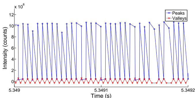
Figure 4.7: Zoom into the peaks and valleys signal recorded by the normalization detector during a full wavenumber scan.
