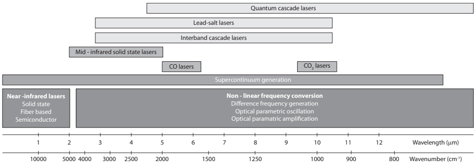
Figure 1.1: Mid-infrared laser sources and their emission regions. The information for this diagram comes from references 34, 49, 50 and 51.
