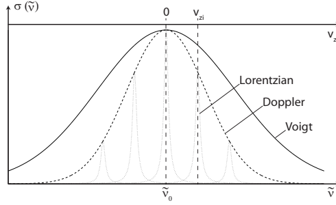
Figure 2.10: Voigt Profile. The inhomogeneous broadening is given by the distribution of the variable v_z , which can be, for example, the speed of the molecules along a given direction.
