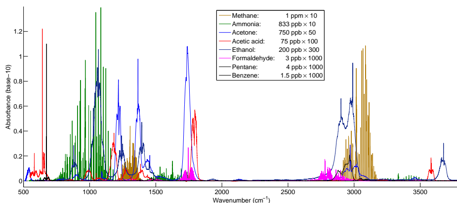
Figure 7.1: Absorbance signature of eight molecules reported in breath after being pre-concentrated. The signal strength corresponds to their average concentration multiply by an adequate enhancement factor. An interaction distance of 54.36 meters is assumed.
