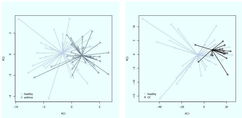
Figure 6.3: Principal component analysis. The dots correspond to the values of the 1 st and 2 nd PCAs and the intersection of the lines shows the average of the PCAs. The subfigure on the left shows the results of comparing the control and asthmatic group. The subfigure on the right corresponds to the comparison between the control and the CF groups.
