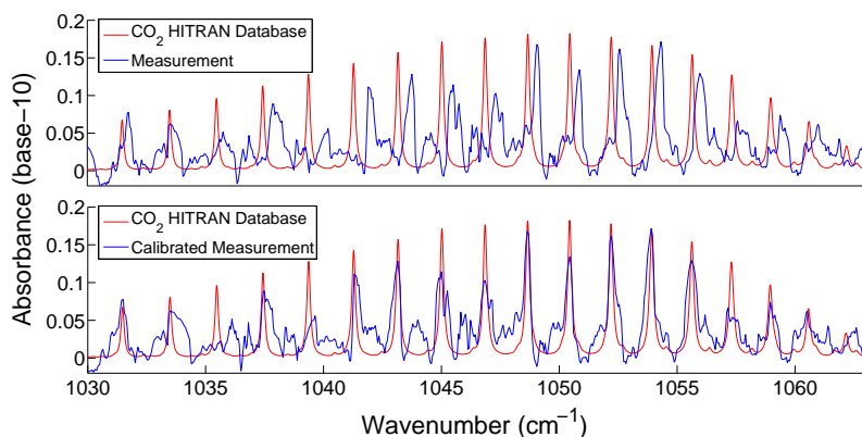
Figure 4.23: Absorbance spectrum obtained with the scan correlation using selected wavenumbers method. The upper plot shows a wavenumber mismatch when compared to the CO 2 absorbance of the HITRAN database. The lower plot shows the calibration applied to the data.
