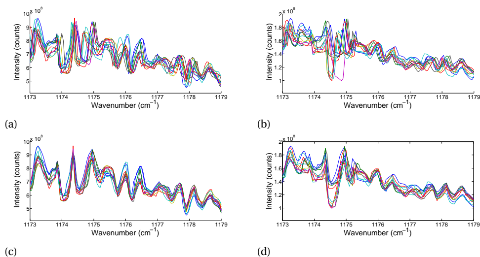
Figure 4.18: Correlation improvement. (a) Uncorrected normalization signals. (b) Uncorrected main signals. (c) Corrected normalization signals. (d) Corrected main signals.
