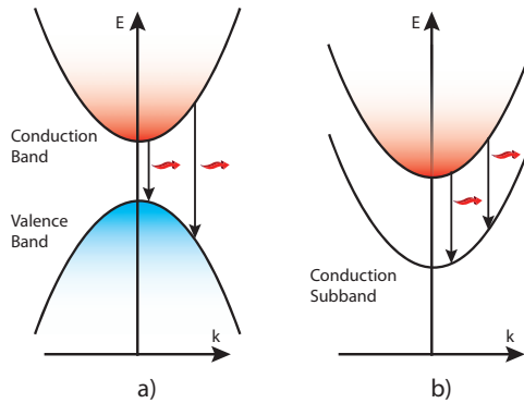
Figure 3.2: Reciprocal space of a) a conventional semiconductor laser and b) the intersubband transitions in a QCL.
