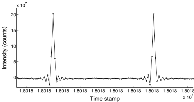
Figure 4.3: Two consecutive pulses recorded by the normalization detector. The circles show the individual data points recorded. 56 points are necessary to capture the 5600 ns period between pulses.
