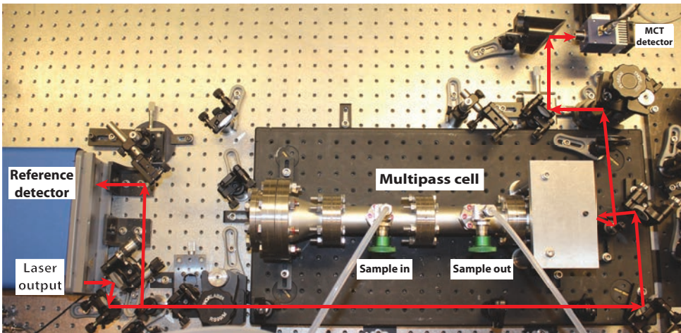
Figure 6.1: Spectroscopic setup.
