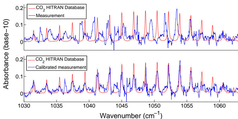
Figure 4.25: Absorbance spectrum obtained with the scan correlation using the STW method. The upper plot shows a wavenumber mismatch when compared to the CO 2 absorbance of the HITRAN database. The lower plot shows the calibration applied to the data.
