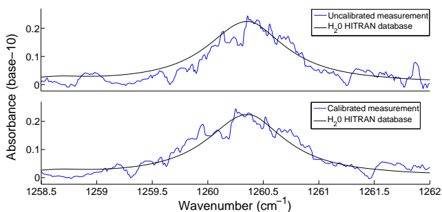
Figure 6.8: Absorption measurement before and after improving the wavenumber calibration using an absorption line of water.
