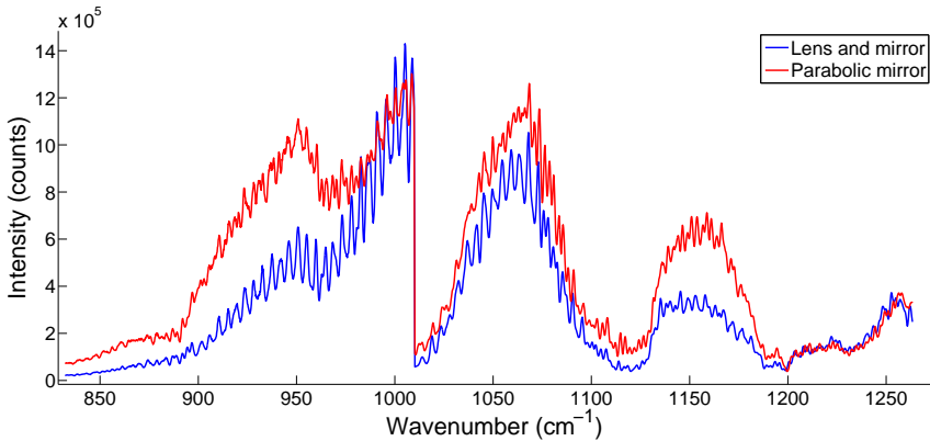
Figure 3.13: QCL spectrum obtained with the normalization detector. The fringes in the blue spectrum are caused by a lens and mirror, which are replaced by a parabolic mirror to obtain the red spectrum.
