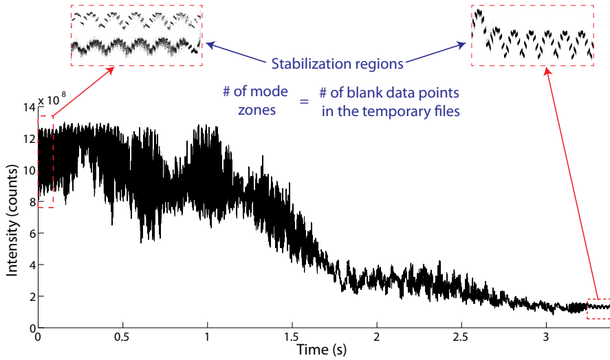
Figure 4.14: Intensity profile of the first QCL obtained with the normalization detector. The stabilization regions are highlighted.
