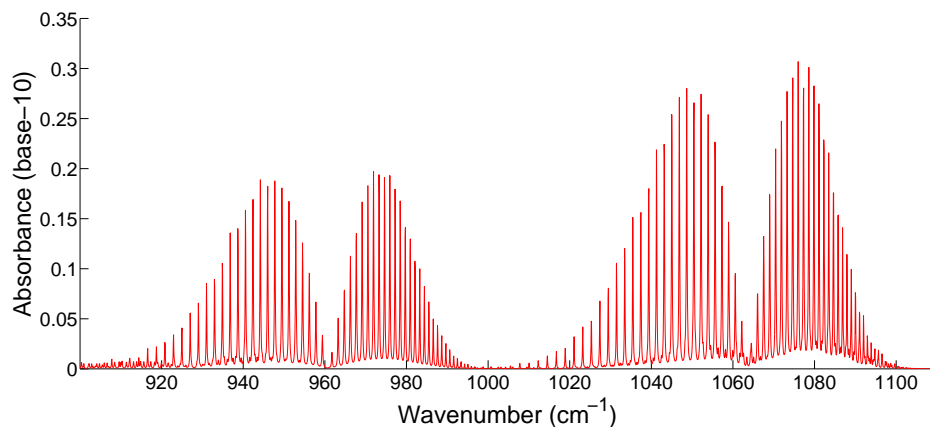
Figure 2.8: Hot bands of \text{CO}_2 . Information from HITRAN database.
