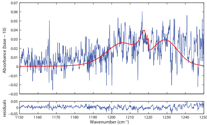
Figure 5.2: Absorbance of acetone with 0.46 \text{ppm}_v concentration after the water lines were removed. The uncertainty is associated to the acetone concentration detection limit of 0.05 \text{ppm}_v ( 1\sigma ). The red line shows the absorbance profile provided by the PNNL database, its strength was found using the multiline fitting routine. The absence of structure in the residuals corroborate that the water removal and the wavenumber calibration are performed correctly.
