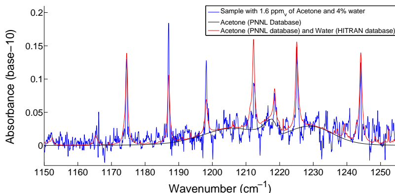
Figure 4.28: Absorbance spectrum of a breath sample with 1.6 ppm v of acetone and 4% water.
