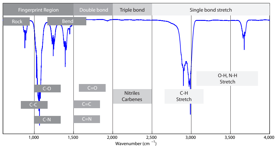
Figure 2.9: Regions where specific bonds induced absorption. Rock and bend refer to two of the different vibration modes of the atoms within a molecule.
