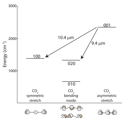
Figure 2.5: Energy level diagram of the vibration modes of CO 2 .
