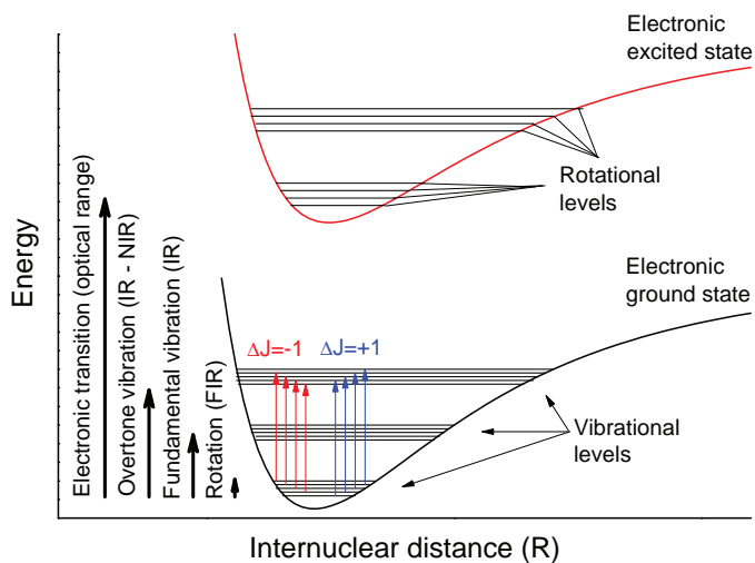
Figure 2.1: Schematic representation of the energy structure of a diatomic molecule. The level of the electric, vibration and rotational energies are in different orders of magnitude. The arrows illustrated transitions between different vibration levels. Reproduced with permission from reference 70
