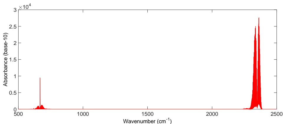
Figure 2.4: Absorption spectrum of \text{CO}_2 . Information from HITRAN database.
