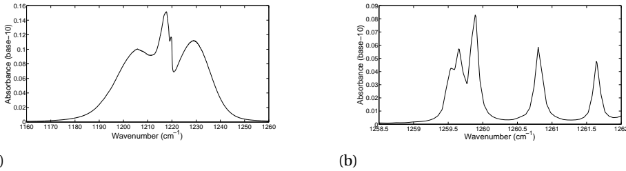
Figure 6.7: Absorption spectrum of (a) acetone and (b) methane. The spectrum of acetone is smooth and covers a broad wavenumber range covering 100\text{ cm}^{-1} . The spectrum of methane consist of sharp absorption lines as point out by the narrow wavenumber range of 3.5\text{ cm}^{-1} presented.
