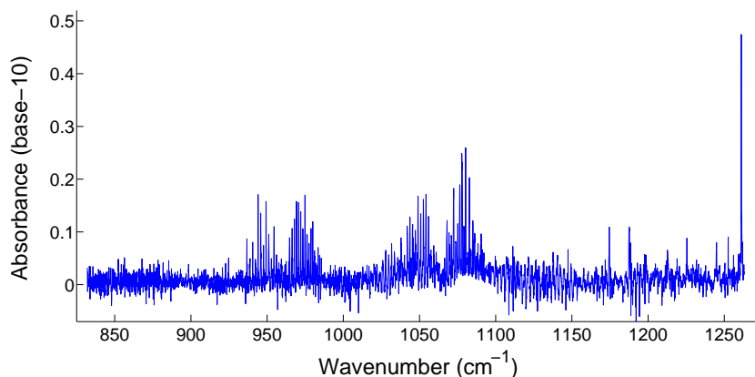
Figure 4.19: Absorbance spectrum of a breath sample built using the selected wavenumber correlation and the wavenumber correction.
