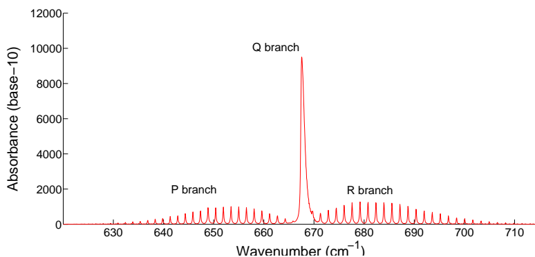
Figure 2.7: P, Q and R branches of the rovibrational spectrum of \text{CO}_2 centered at 667 \text{ cm}^{-1} . Information from HITRAN database.
