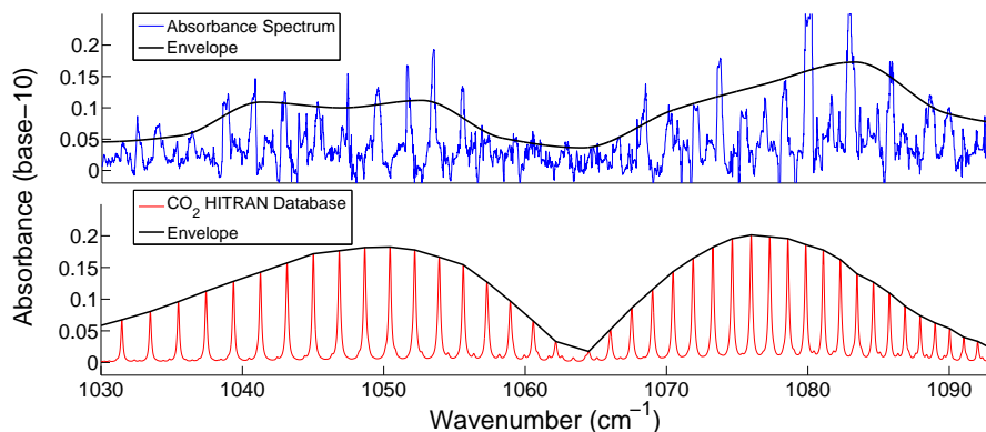
Figure 4.24: Rough calibration of the absorbance spectrum obtained with the scan correlation using the STW method. The upper plot shows the data measurement and its envelope. The lower plot shows the \text{CO}_2 absorbance of the HITRAN database and its envelope.
