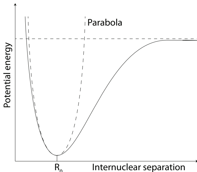
Figure 2.2: Schematic representation of the potential of a diatomic molecule.
