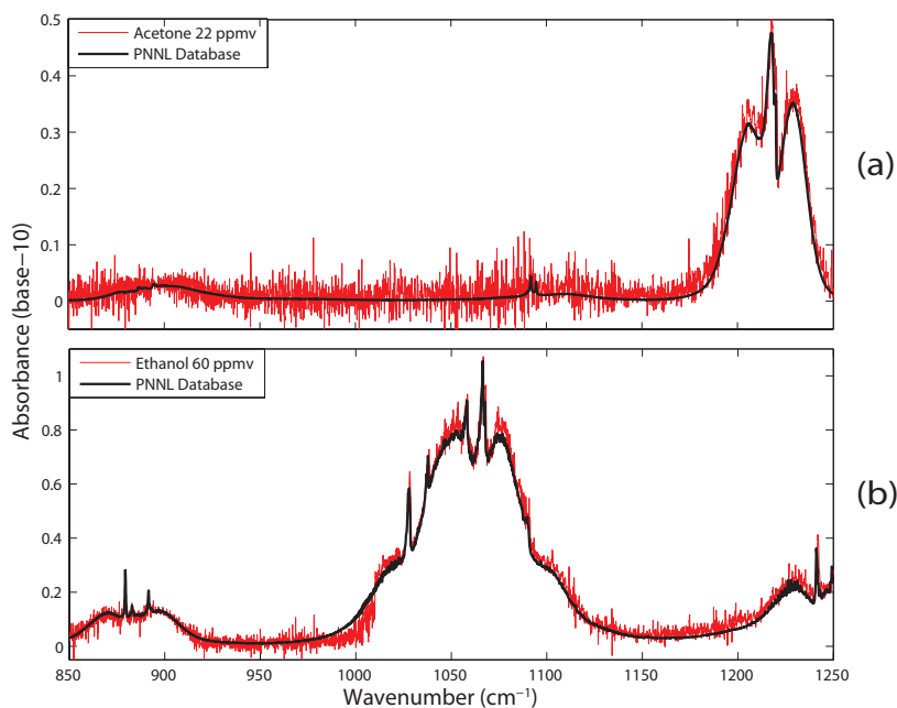
Figure 3.15: Absorption spectrum of 22 ppm v of acetone and 60 ppm v of ethanol. Both at 900 mbar in an atmosphere of N 2 .
