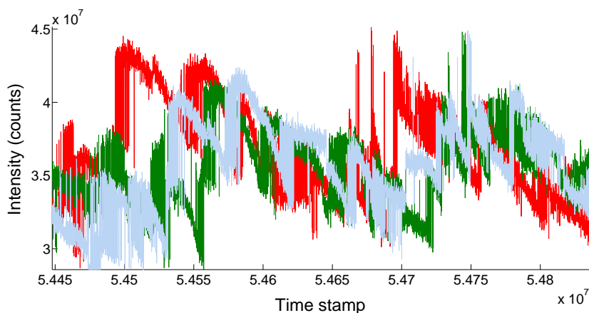
Figure 4.10: Mismatch in the intensity profile of three consecutive wavenumber scans.
