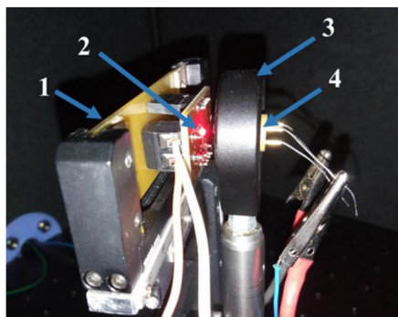
Figure 7. Optical setup for irradiance measurements. (1) LED holder, (2) LED, (3) photodiode holder, and (4) Thorlabs FDS 100-CAL Si calibrated photodiode.
