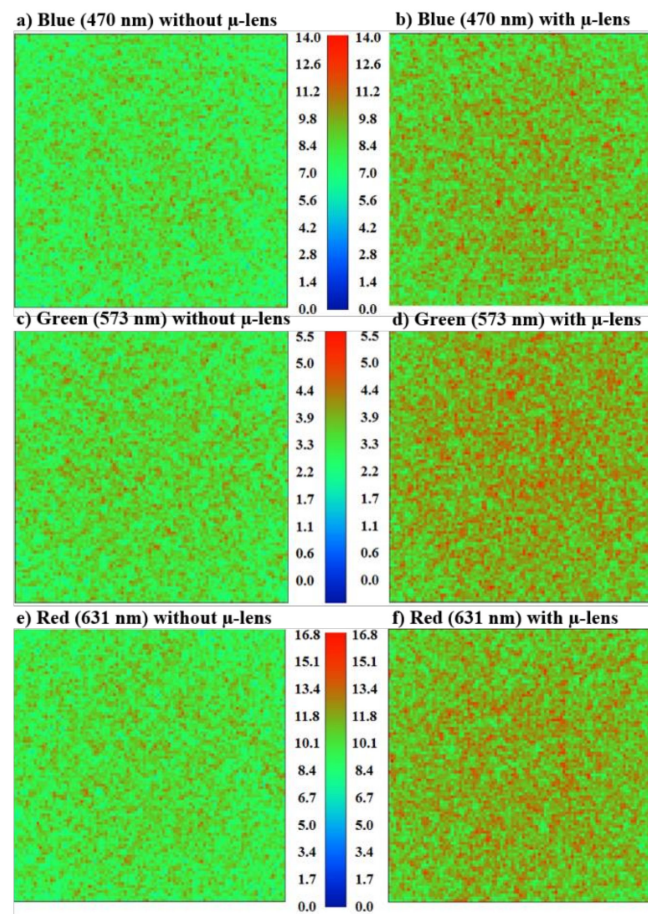
Figure 3. ZEMAX® irradiance maps simulation results for: blue LED (a) without \mu -lens and (b) with \mu -lens; green LED (c) without \mu -lens and (d) with \mu -lens; and red LED (e) without \mu -lens and (f) with \mu -lens.
