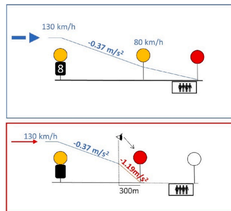
Fig. 4. Hypothetical example where the standard situation with a deceleration of 0.37 \text{ m/s}^2 is sufficient. If the train driver employs the same amount of deceleration during the green-yellow-red approach, then this insufficient deceleration can be corrected if, upon seeing the red aspect at 300 m, the train can decelerate by at least 1.19 \text{ m/s}^2 continuously.
