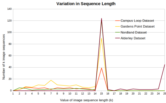
FIGURE 6. The variation in sequence length of ConvSequential-SLAM on all four datasets is shown here.
