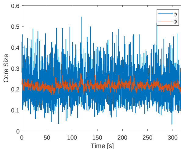
Figure 22. Core size obtained for an air flow rate of 110 L/min and a water flow rate of 113 L/min at fixed valve positions, which maximize \eta_m . In blue: original ERT signal. In orange: output of the low-pass filter ( \omega_f = 1 rad/s). Signals with standard deviation \sigma(y) = 0.0724 and \sigma(\hat{y}) = 0.0146 .
