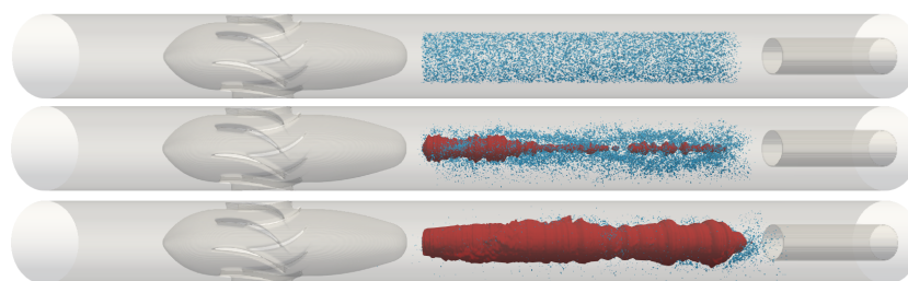
Figure 20. Simulation performed using the hybrid Lagrangian tracking–volume of fluid solver. The blue dots correspond to bubbles, and the red region corresponds to the coalesced core. ( Top ) t = 0 s (initial condition); ( Middle ) t = 0.011 s; ( Bottom ) t = 0.040 s.
