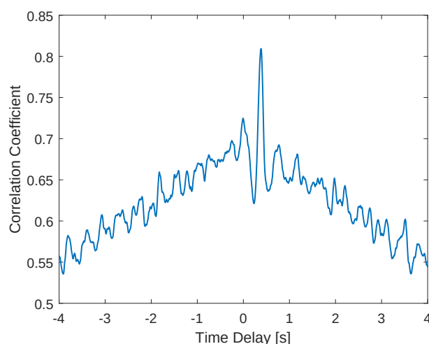
Figure 17. Cross-correlation coefficient between the camera and wire-mesh sensor volumetric fractions of air for a liquid flow rate of 160 L/min and an air flow rate of 170 L/min.
