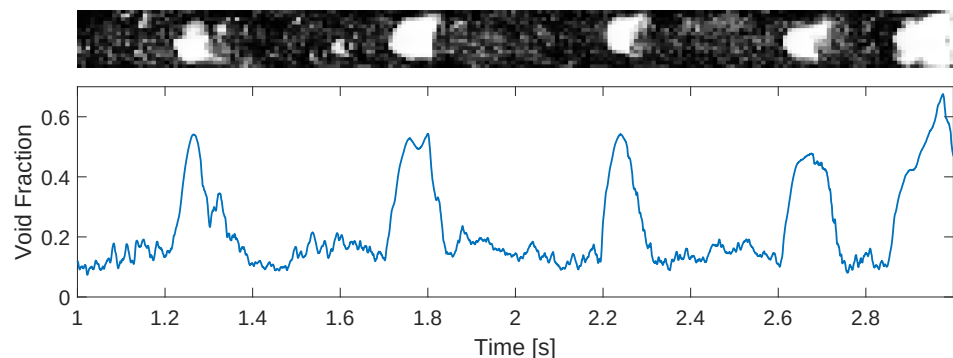
Figure 13. Gas–liquid distribution ( top ) and volumetric fraction of air ( bottom ) of a slug flow measured by the wire-mesh sensor installed upstream of the ISS for a water flow rate of 80 L/min and an air flow rate of 70 Ln/min. The two images correspond to the same data and share the same time axis. Gas is represented in white and liquid in black in the images, with the light intensity of gray pixels proportional to the local gas fraction measured by the WMS.
