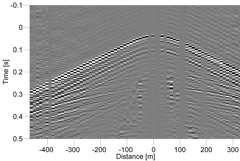
Figure 2.10: Seismic records obtained at 50-m depth with a 10-s linear sweep from 5 to 200 Hz. Vertical-geophone data shown in panel (a), Hydrophone data shown in panel (b). (Dead traces are blanked.)
