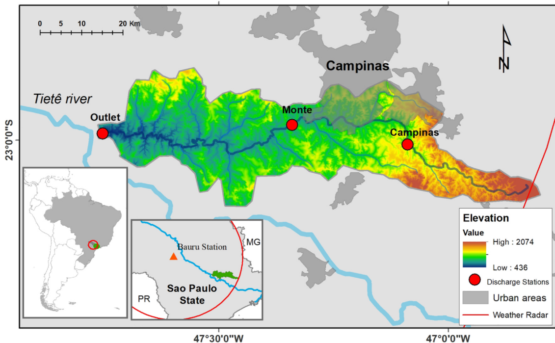
Fig. 2. Geographical location of the Capivari catchment. Red dots represent the discharge station of Campinas, Monte and the virtual station in Outlet. Red cycled represent the weather radar Bauru used as ground measurements. (For interpretation of the references to colour in this figure legend, the reader is referred to the web version of this article.)
