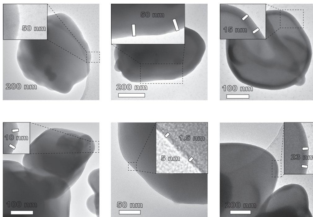
Fig. 2. TEM images of budesonide particles, uncoated and coated by \text{SiO}_2 , \text{Al}_2\text{O}_3 and \text{TiO}_2 films via ALD, by poly(ethylene) terephthalate films via MLD and by titaniconic films via \text{TiCl}_4/\text{EG} hybrid ALD/MLD. The deposition processes of \text{Al}_2\text{O}_3 , \text{TiO}_2 , PET and titaniconic were run for 50 cycles, whereas that of \text{SiO}_2 for 100 cycles. The details of the experimental conditions are reported in Table S1. The film thicknesses were measured by ImageJ.
